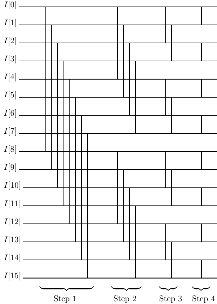
Figure 1. Batcher's bitonic merger for n = 16 elements
