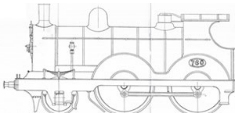
3 1/2" 2-4-0 Gauge GER Tender Locomotive by L.B.S.C.
