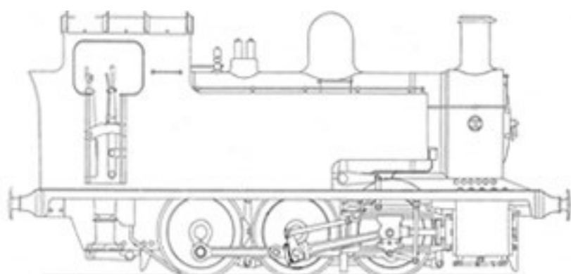
5" Gauge 0-6-0 Tank Locomotive by Charles Kennion
