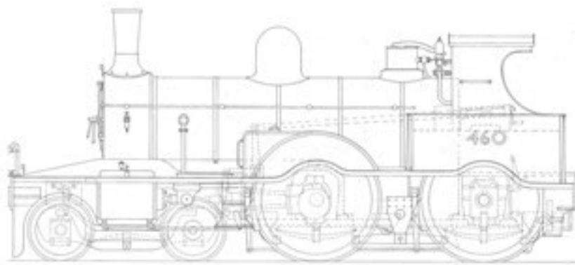
5" Gauge 4--4-0 LSWR 460 Class W Adams 1884 Tender Locomotive
