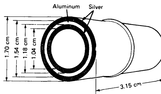
Fig. 2 The low-susceptibility proof-mass design.
