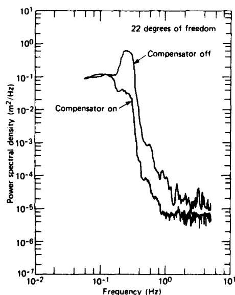
Fig 2 Depth power spectral density for compensator on and compensator off with the CTD profiler kept at a fixed cable length.
