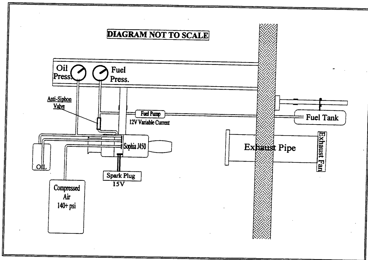
Figure 7. Building 216 Engine Test Rig.
