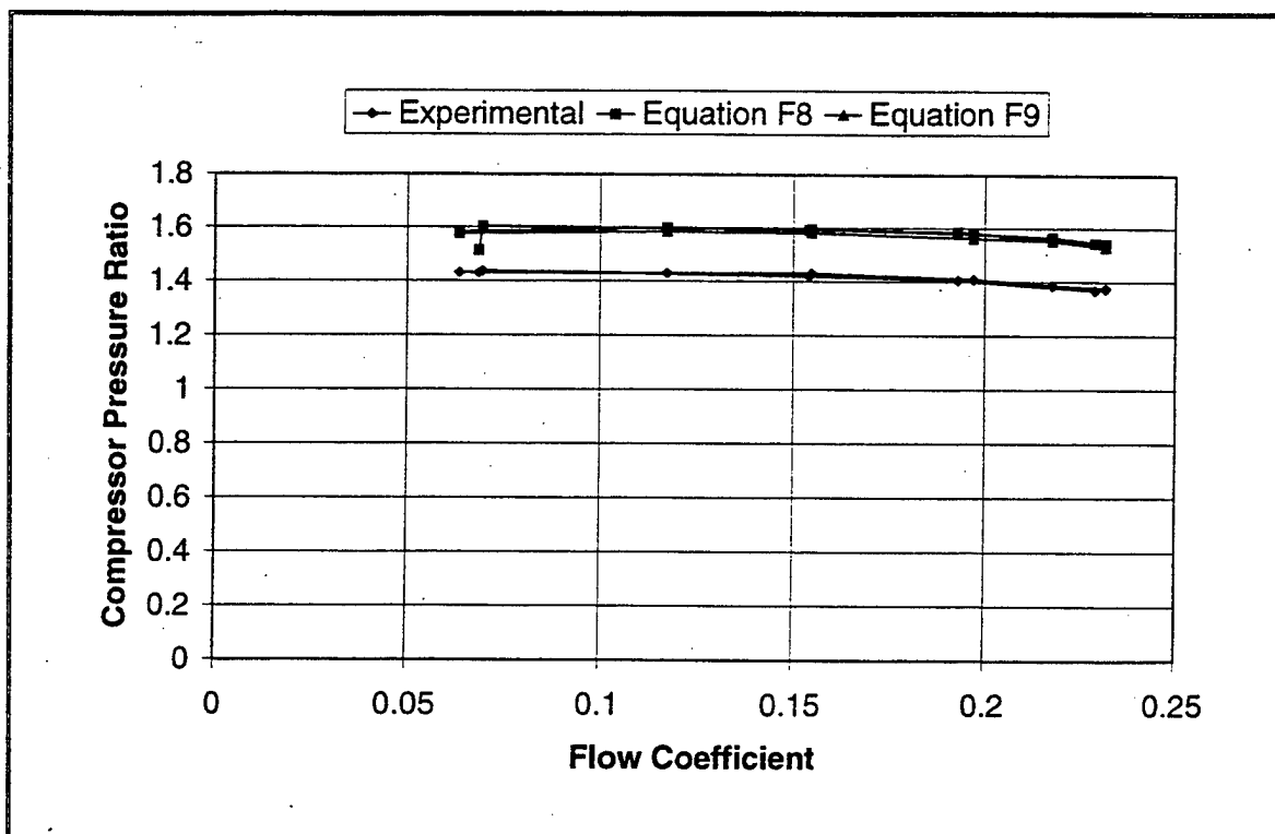
Figure F5. Garrett T2 Turbocharger Compressor Pressure Ratio (100,000 RPM).
