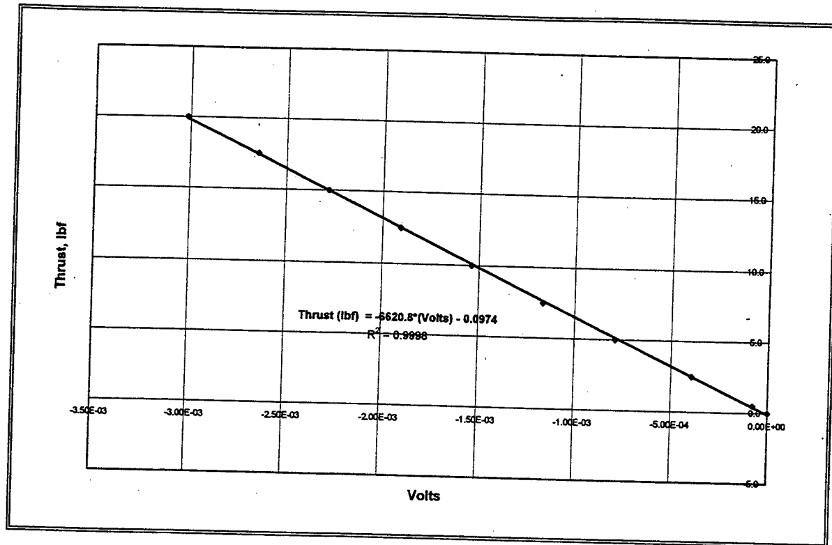
Figure C1. Sophia J450 Test Program Thrust Beam Calibration Curve.
