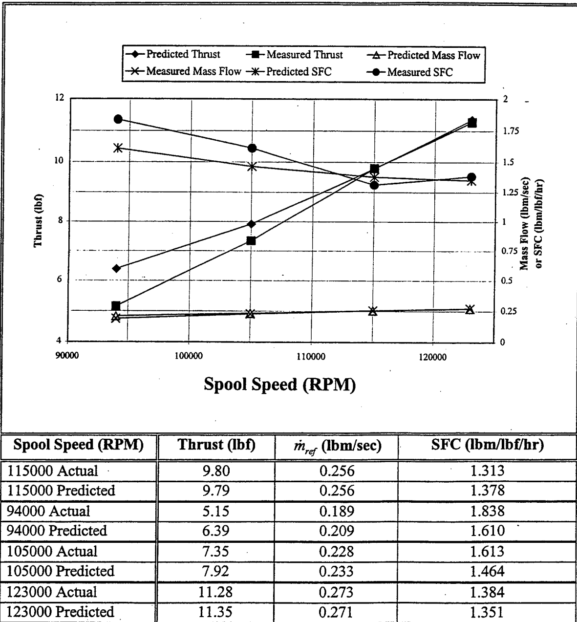
Figure 10. GASTURB Prediction vs Actual Sophia J450 Performance.
