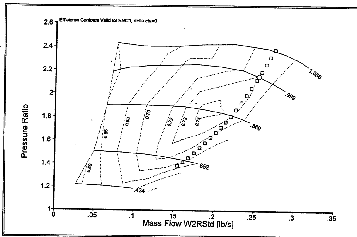
Figure 11. GASTURB-Predicted Sophia J450 Compressor Operating Line.
