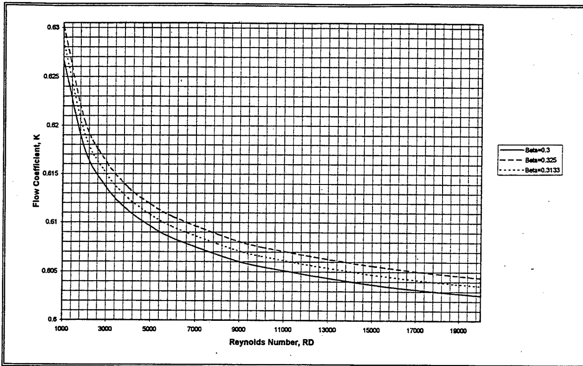
Figure B2(a). Flow Coefficient, K , as a Function of Pipe Reynolds Number and Diameter Ratio, \beta , for 6.065 in. Diameter Pipe, After Ref. [5].
