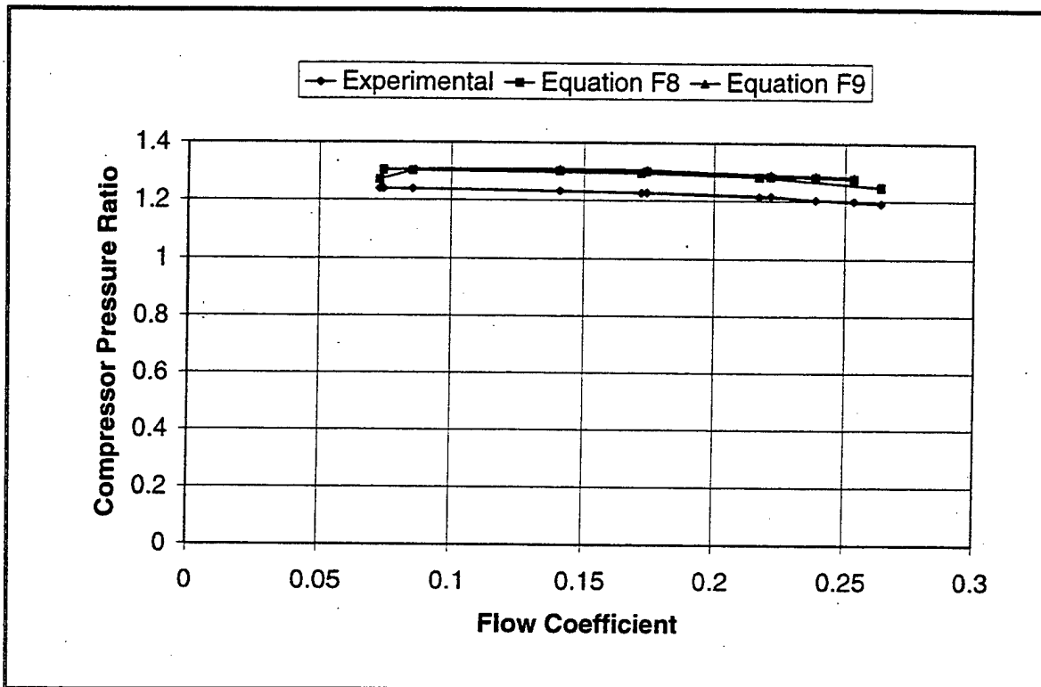
Figure F4. Garrett T2 Turbocharger Compressor Pressure Ratio (75,000 RPM).
