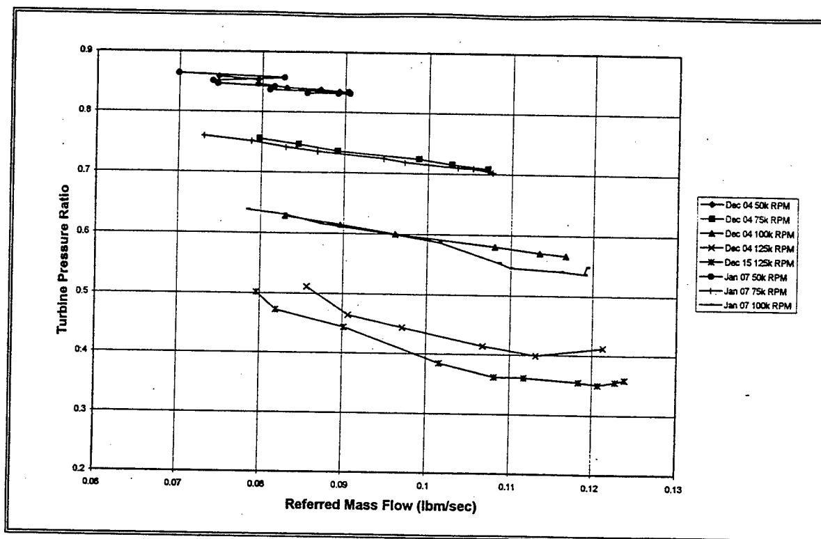
Figure A1. Garrett T2 Turbocharger Turbine Total-to-Total Pressure Ratio vs Referred Mass Flow Rate.
