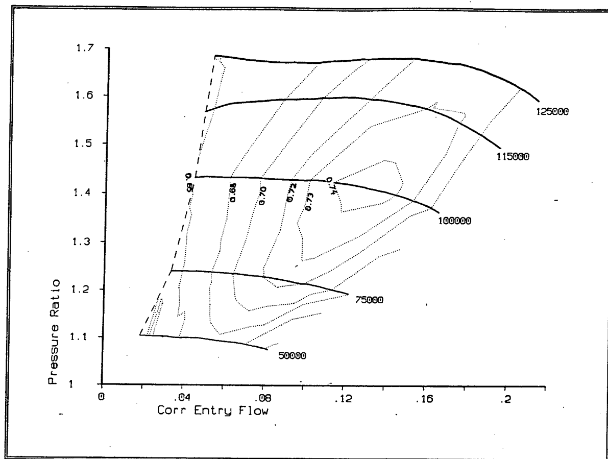
Figure 9. Garrett T2 Turbocharger Compressor SMOOTHC Performance Map.
