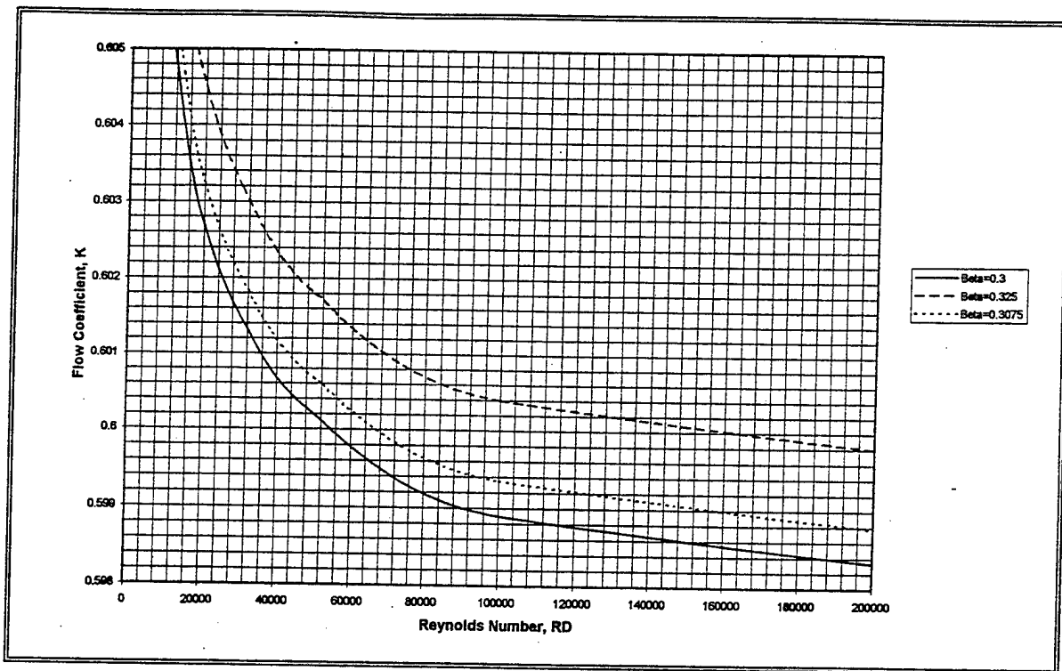
Figure B1(c). Flow Coefficient, K , as a Function of Pipe Reynolds Number and Diameter Ratio, Beta , for 4.026 in. Diameter Pipe, After Ref. [5].
