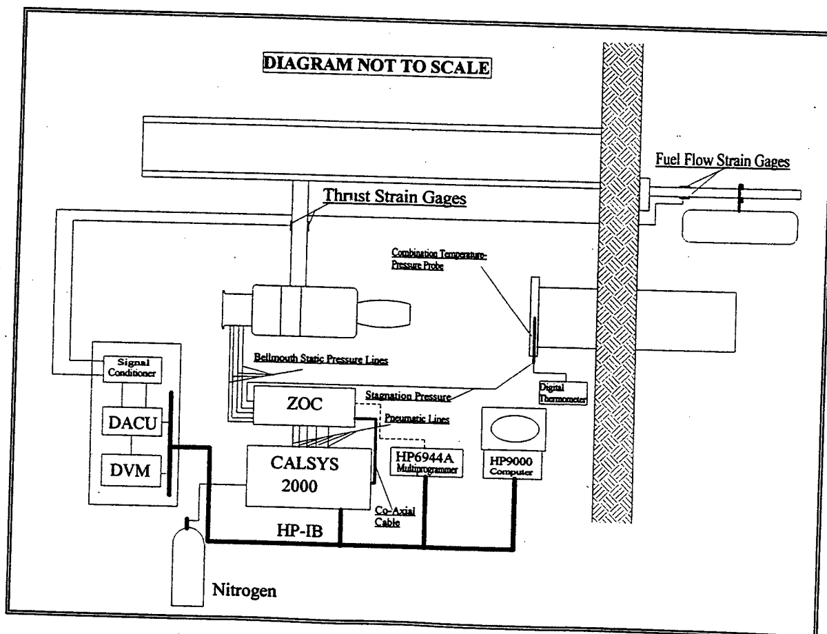
Figure 8. Engine Test Rig Data Acquisition Schematic.
