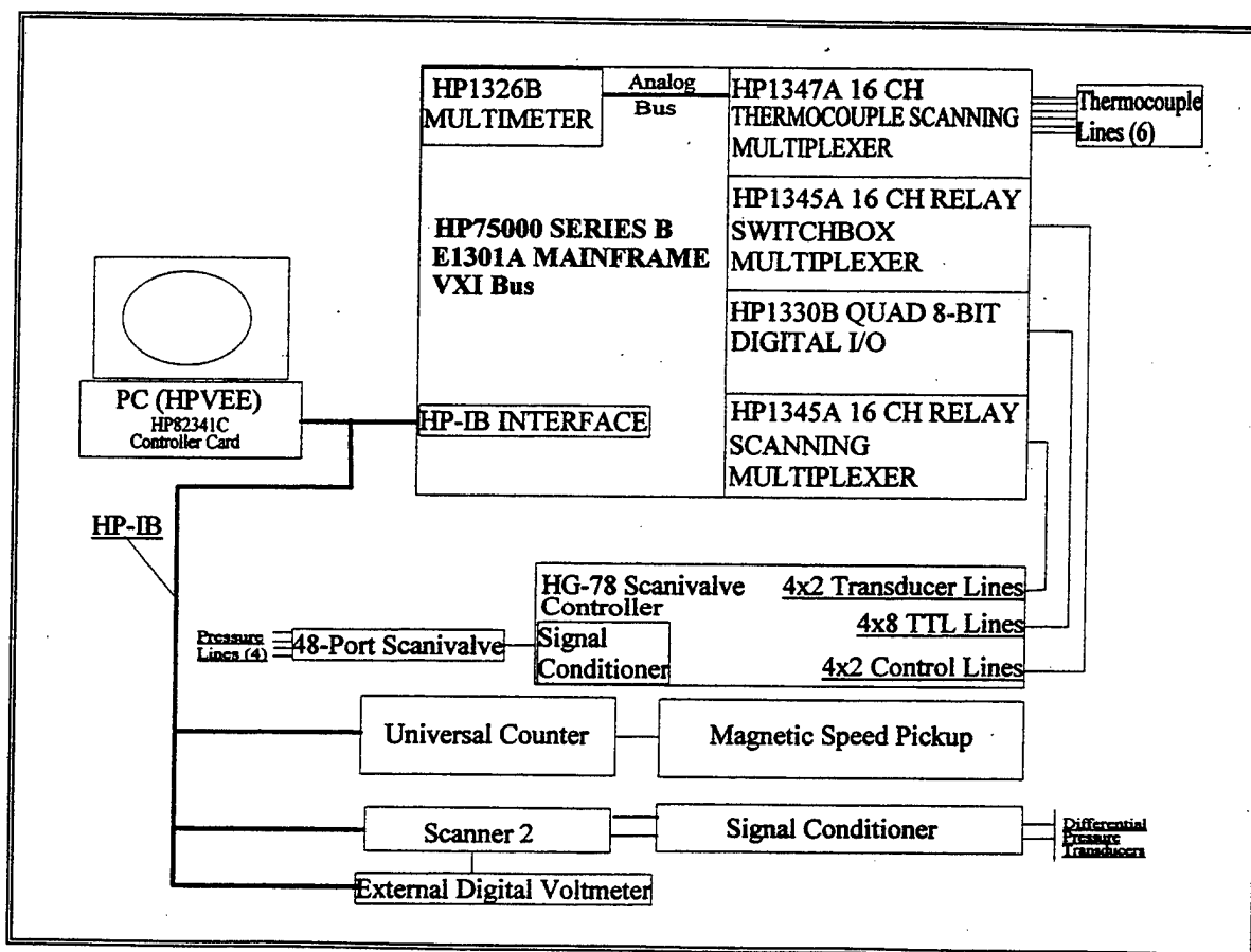
Figure 3. Turbocharger Data Acquisition Schematic.
