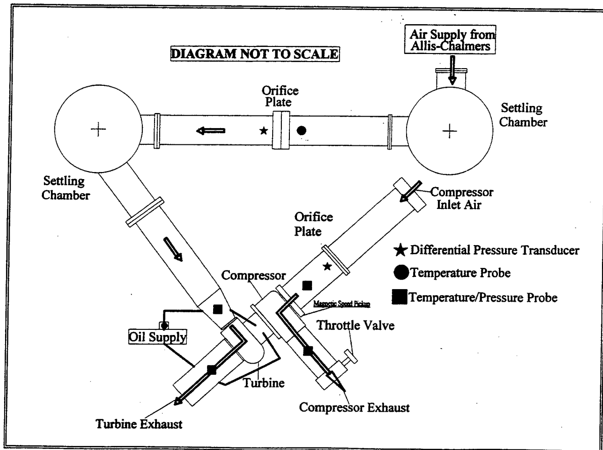
Figure 2. Turbocharger Test Rig Layout.
