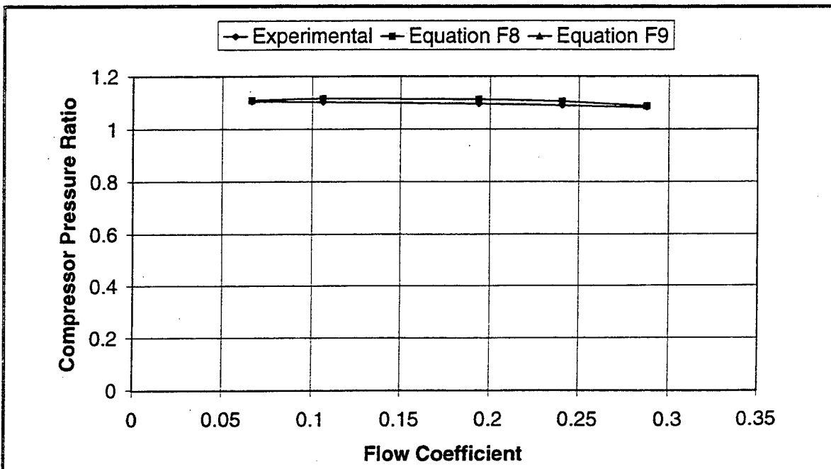
Figure F3. Garrett T2 Turbocharger Compressor Pressure Ratio (50,000 RPM).
