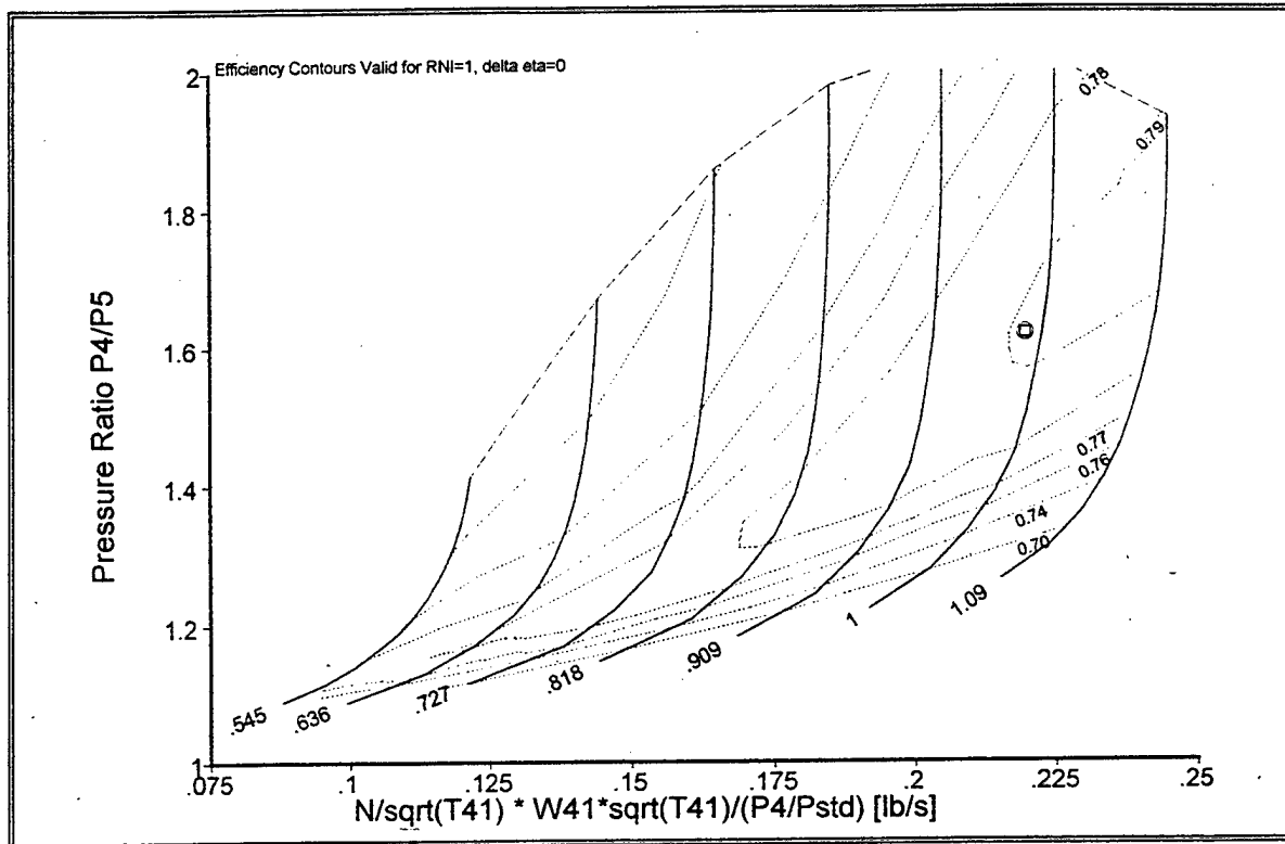
Figure E3. GASTURB Default Turbine Performance Map.
