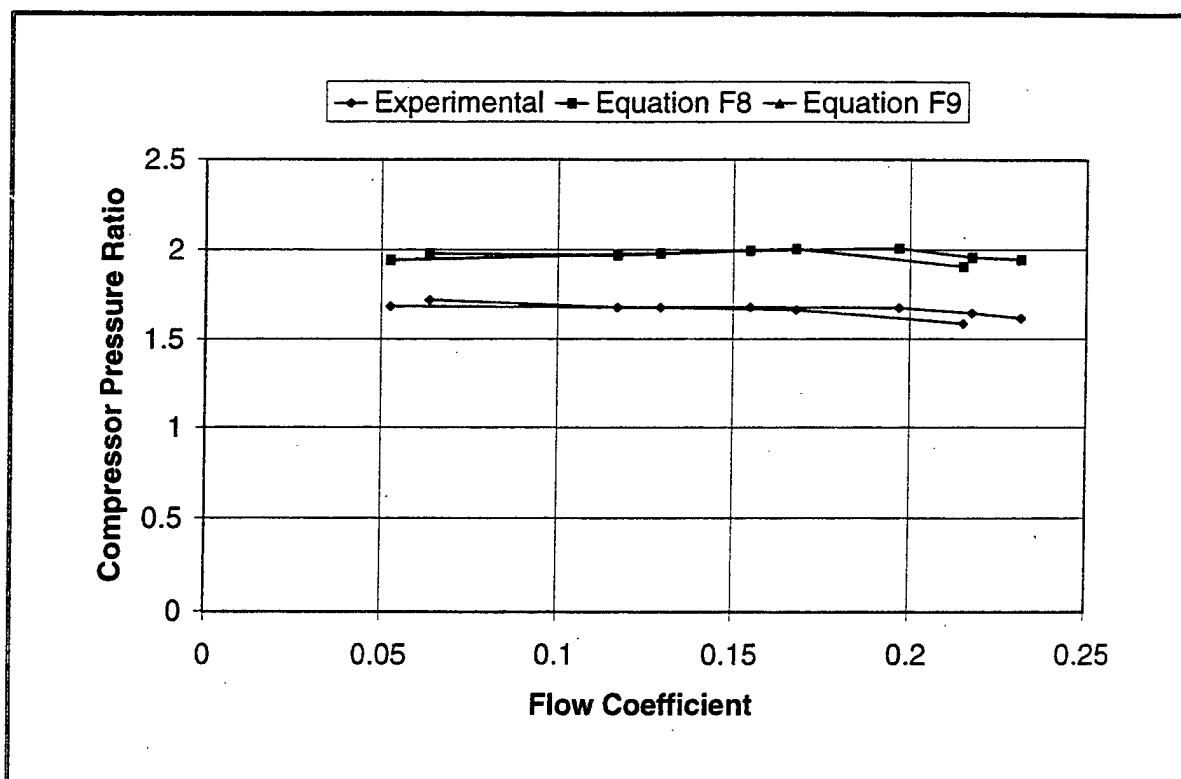
Figure F6. Garrett T2 Turbocharger Compressor Pressure Ratio (125,000 RPM).
