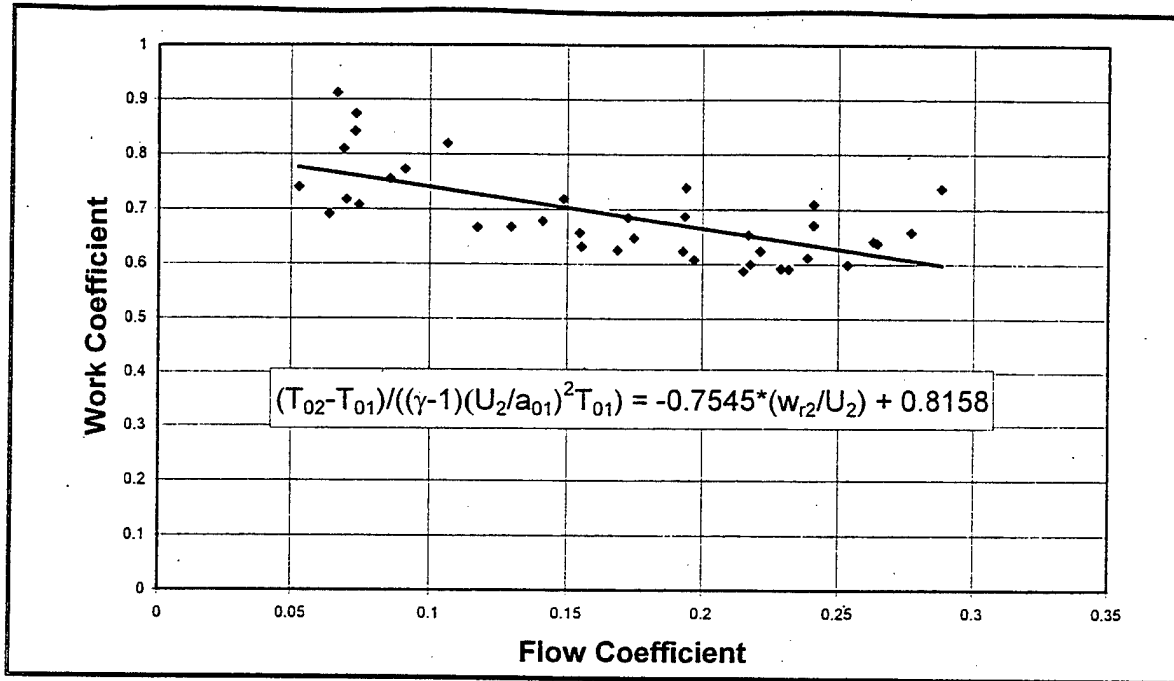
Figure F1. Work Coefficient Characteristic of the Garrett T2 Compressor.
