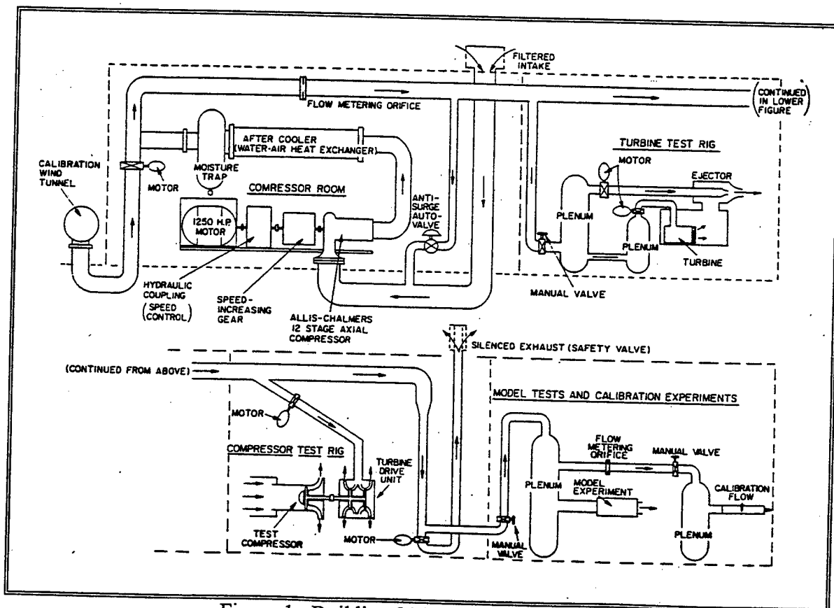
Figure 1. Building 215 Air Supply System.
