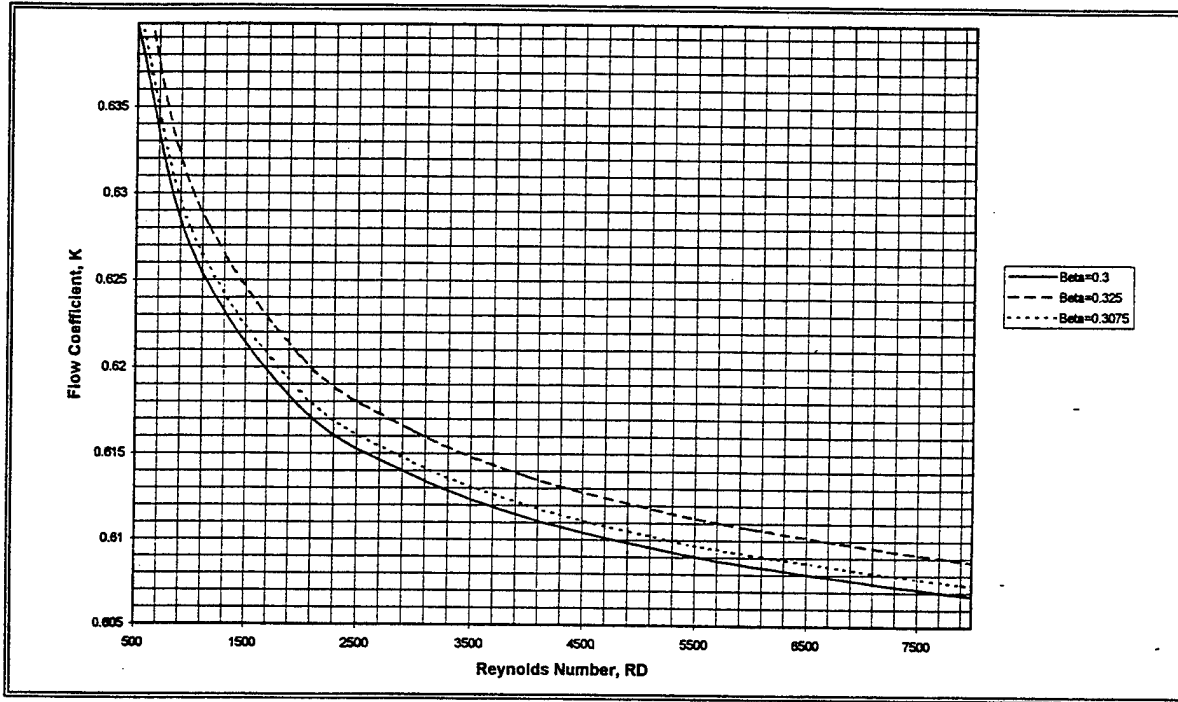
Figure B1(a). Flow Coefficient, K , as a Function of Pipe Reynolds Number and Diameter Ratio, \beta , for 4.026 in. Diameter Pipe, After Ref. [5].
