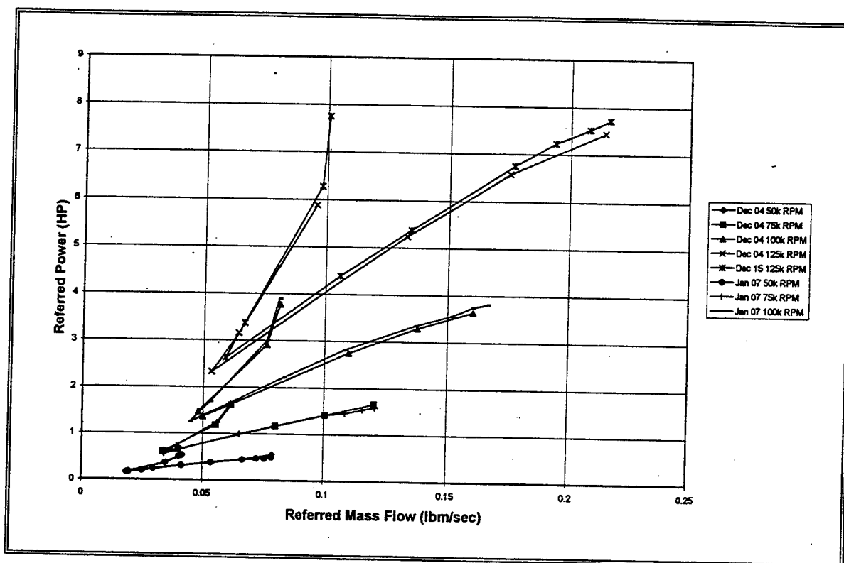
Figure 6. Garrett T2 Turbocharger Compressor Referred Power vs Referred Mass Flow Rate.
