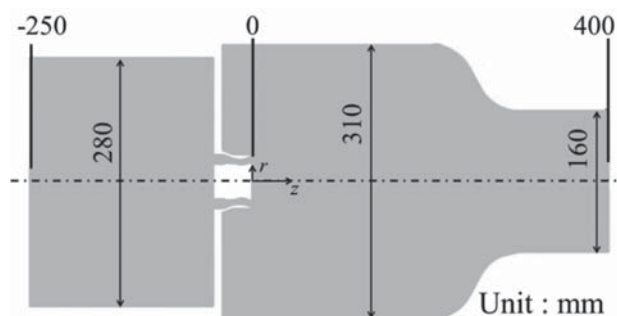
Fig. 7 Computational domain for LES.
