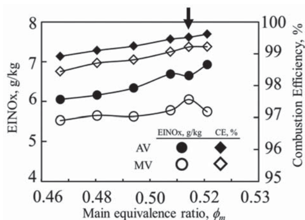
Fig.15 Effects of relative position of swirl vanes to fuel injection holes on NOx emission indices and combustion efficiency.
