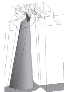
(c) Rotor blade shape
