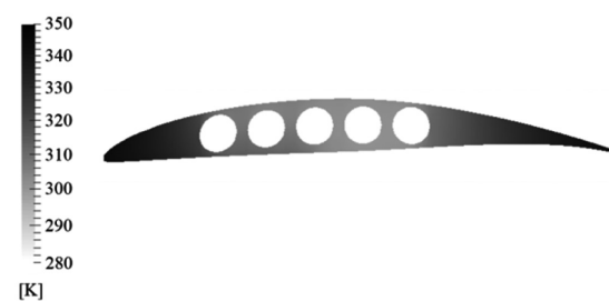
(a) Inverse heat conduction method
