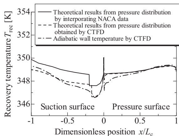
Fig. 11 Comparison of recovery temperature from pressure distributions obtained by interpolating NACA data and CTFD with adiabatic wall temperature obtained by CTFD
