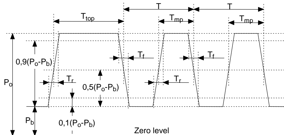
Figure 17 - Write pulse
