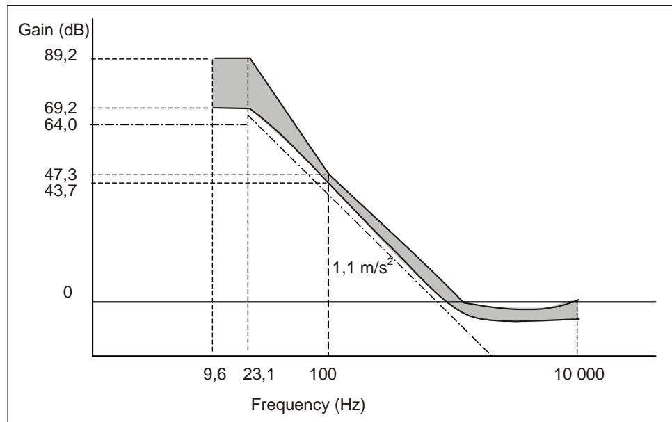
Figure 5 - Reference servo for radial tracking
