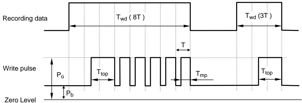
Figure 16 - Basic write strategy
