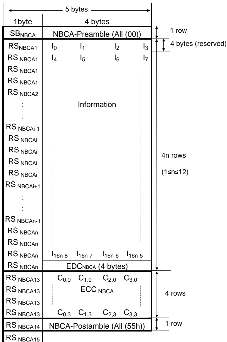
Figure L.2 - NBCA-Data structure
