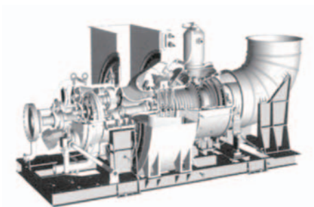
図6 Orenda Aerospace社製OGT2500
