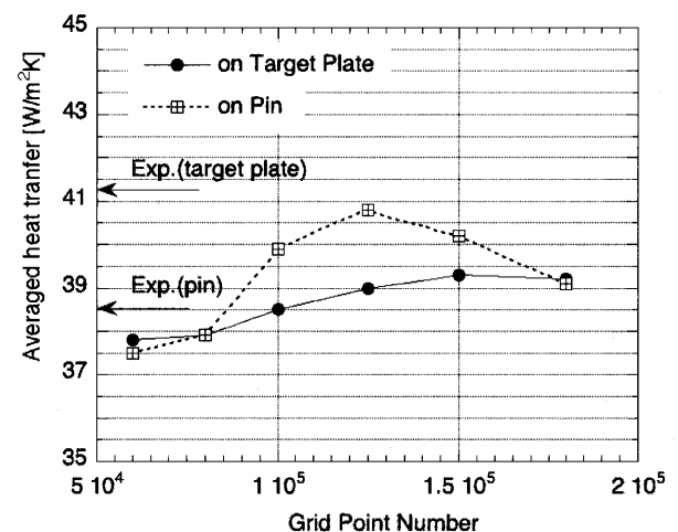
Fig.6 Variations of averaged heat transfer coefficients with grid point number
