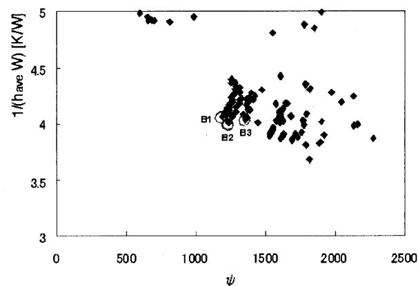
Fig. 11 Pareto optimum solutions for case 3
