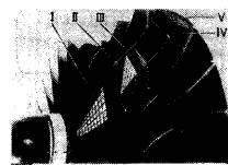
Fig. 2 Centrifugal compressor impeller with arrangement of optical measurement areas in the blade channels (impeller blackened by anodic treatment to reduce background radiation)
