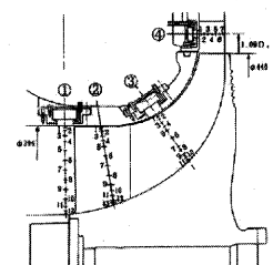
Fig. 15 LDF Measuring Sections
