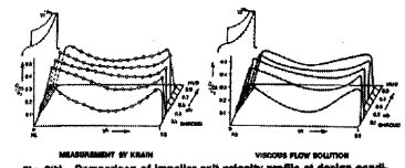
Fig. 7 Comparison of impeller exit velocity profile at design condition ( Re = 1, M = 4 )
