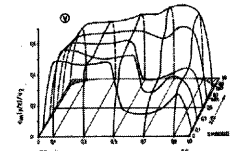
Fig. 4 Velocity distribution u, v, w at measurement area Re = 14,000
