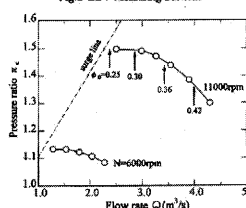
Fig. 16 Compressor Characteristics
