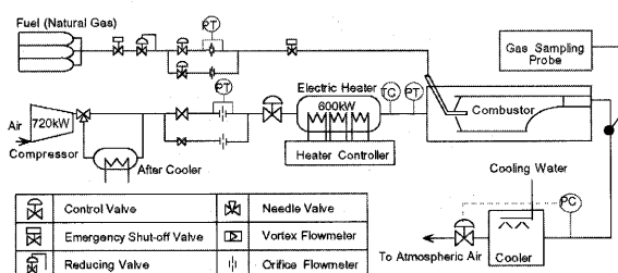
Fig.6 Pressurized test facility
