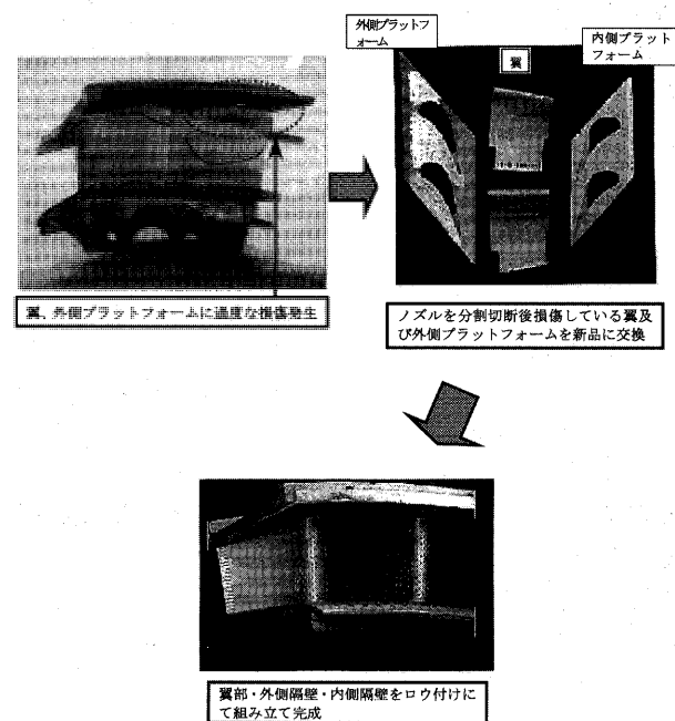
図8 Airfoil Replacement
