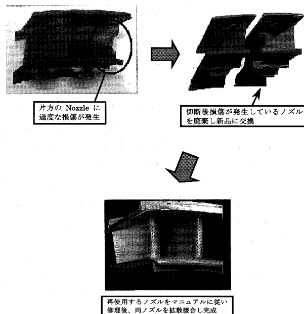
図7 Split Vane Replacement
