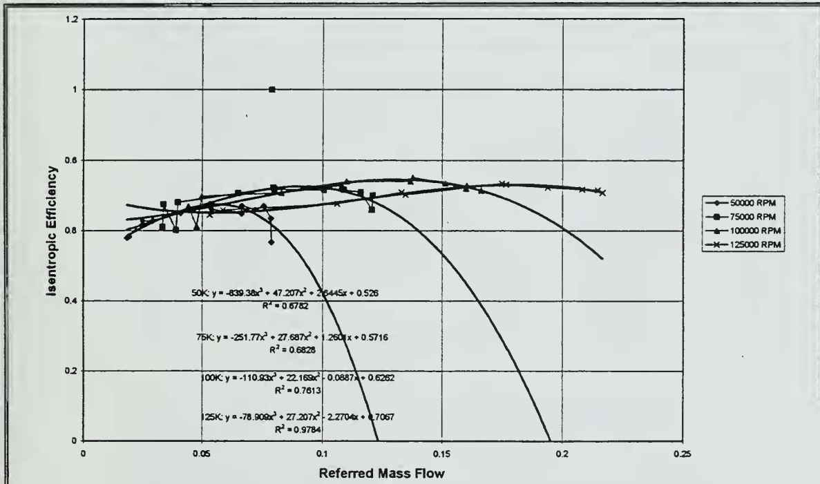
Figure E2. Garrett T2 Compressor Efficiency Map (Trimmed and Fitted).
