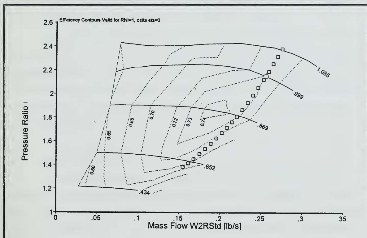
Figure 11. GASTURB-Predicted Sophia J450 Compressor Operating Line.
