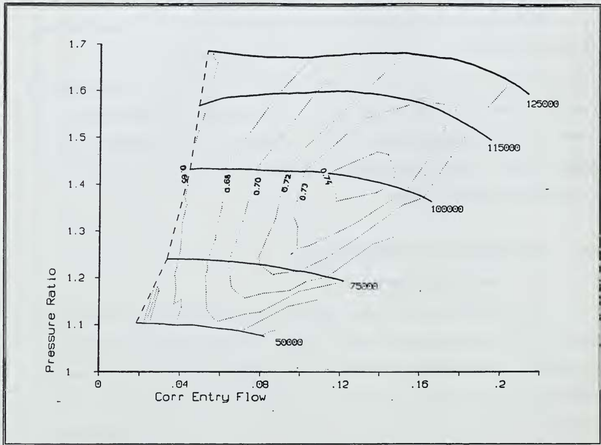
Figure 9. Garrett T2 Turbocharger Compressor SMOOTHC Performance Map.
