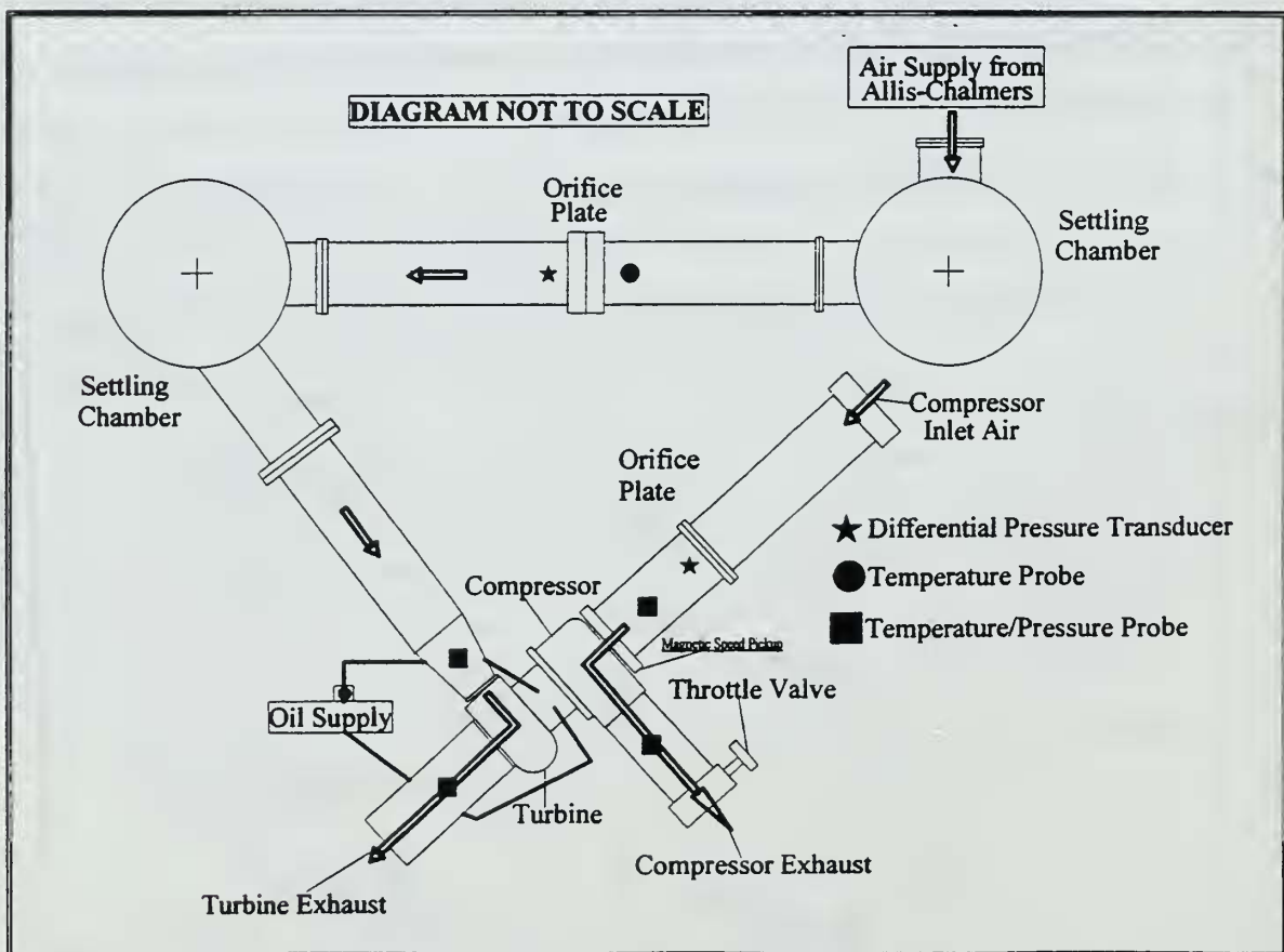
Figure 2. Turbocharger Test Rig Layout.
