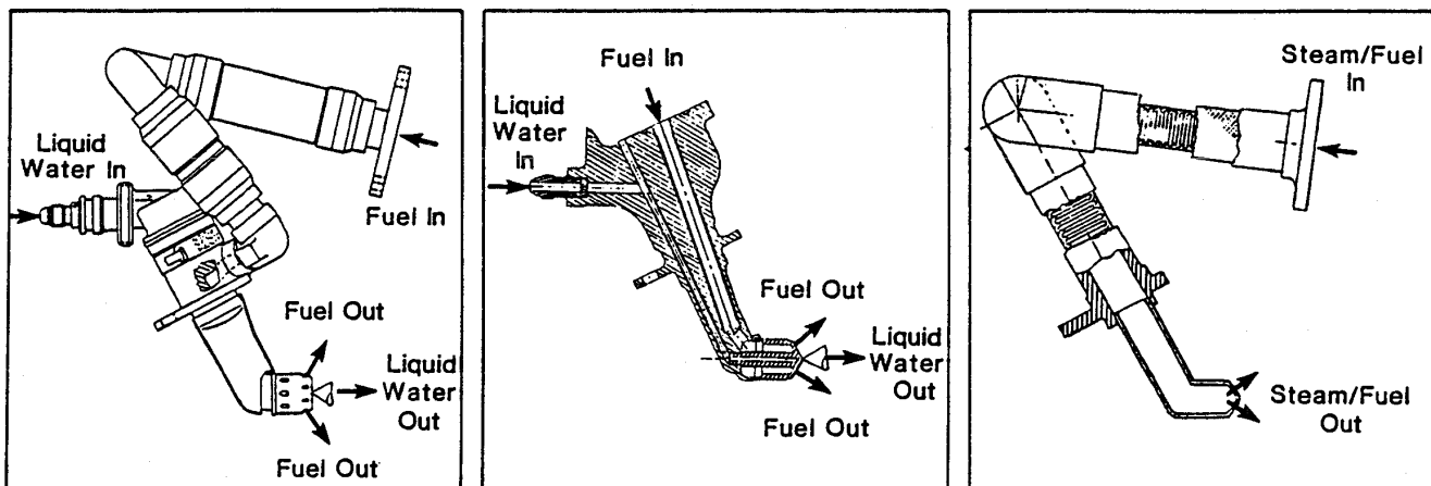
Water Injection Methods Evaluated In LM2500 and LM5000 Combustor Component Tests With Natural Gas Fuel
