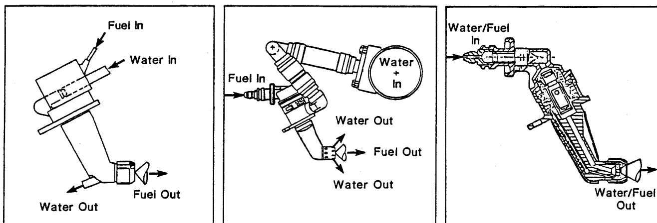
Liquid Water Injection Methods Evaluated In LM2500 Combustor Component Tests With Diesel Fuel
