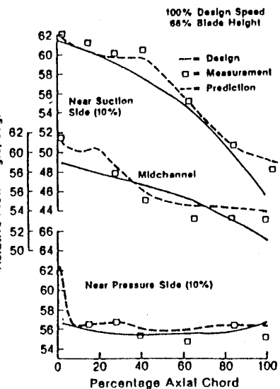
Comparison of relative flow angle distribution at maximum efficiency ( m = 17.15 \text{ kg/s} ).
