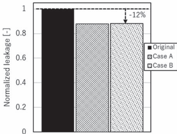
Fig. 11 Leakage performance
