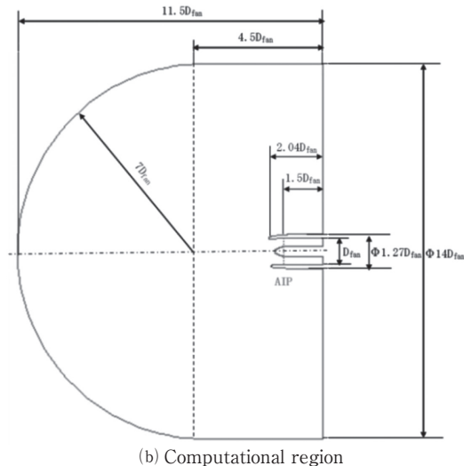
Fig. 3 Computational model
