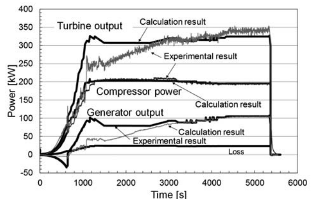
Fig. 9 Power histories
