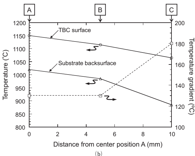
Fig. 3 (a) TBC surface and substrate backsurface temperature at position A during thermal cycling. (b) Temperature gradient at position A, B and C indicated in Fig. 2.
