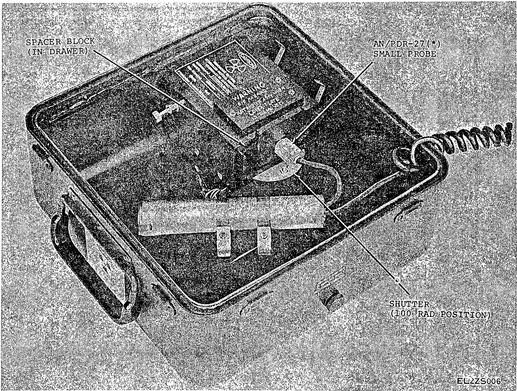
Figure 3-2 checking AN/PDR-27(*) on 500 mrad/hr range
