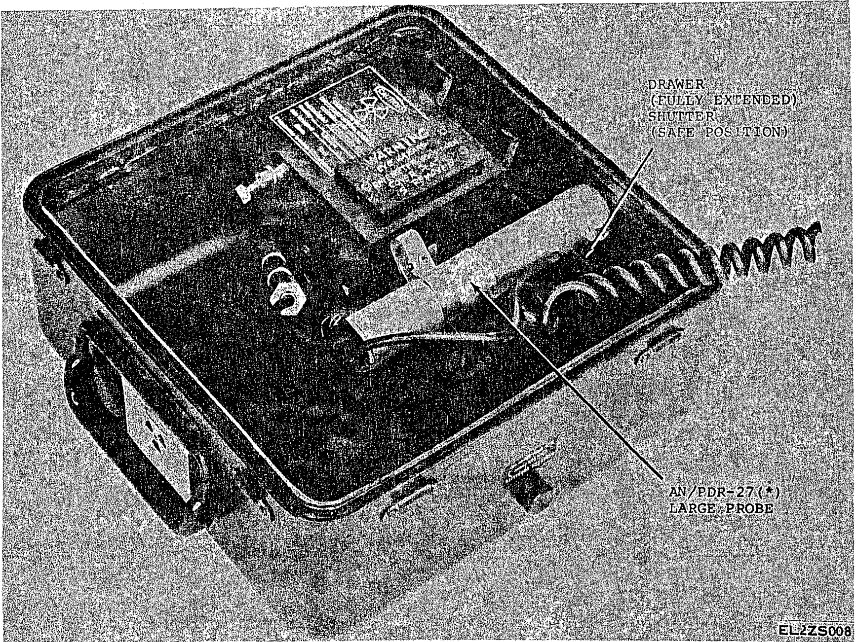
Figure 3-4. Checking AN/PDR-27(*) on 5 mrad/hr range.
