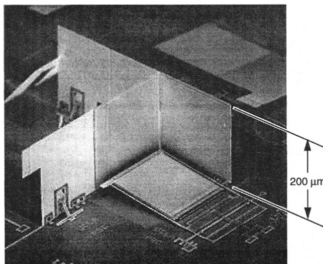
Figure 2. Microfabricated corner-cube retroreflector, consisting of three gold-coated polysilicon mirrors. The base mirror can be deflected electrostatically, modulating the optical signal reflected from the device (taken from [2]).
