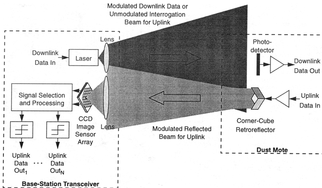
Figure 3. Design of a free-space optical network in which a base-station transceiver communicates simultaneously with a collection of many dust motes (only one dust mote is shown). A single laser at the base station supplies optical power for the downlink and the uplink.
