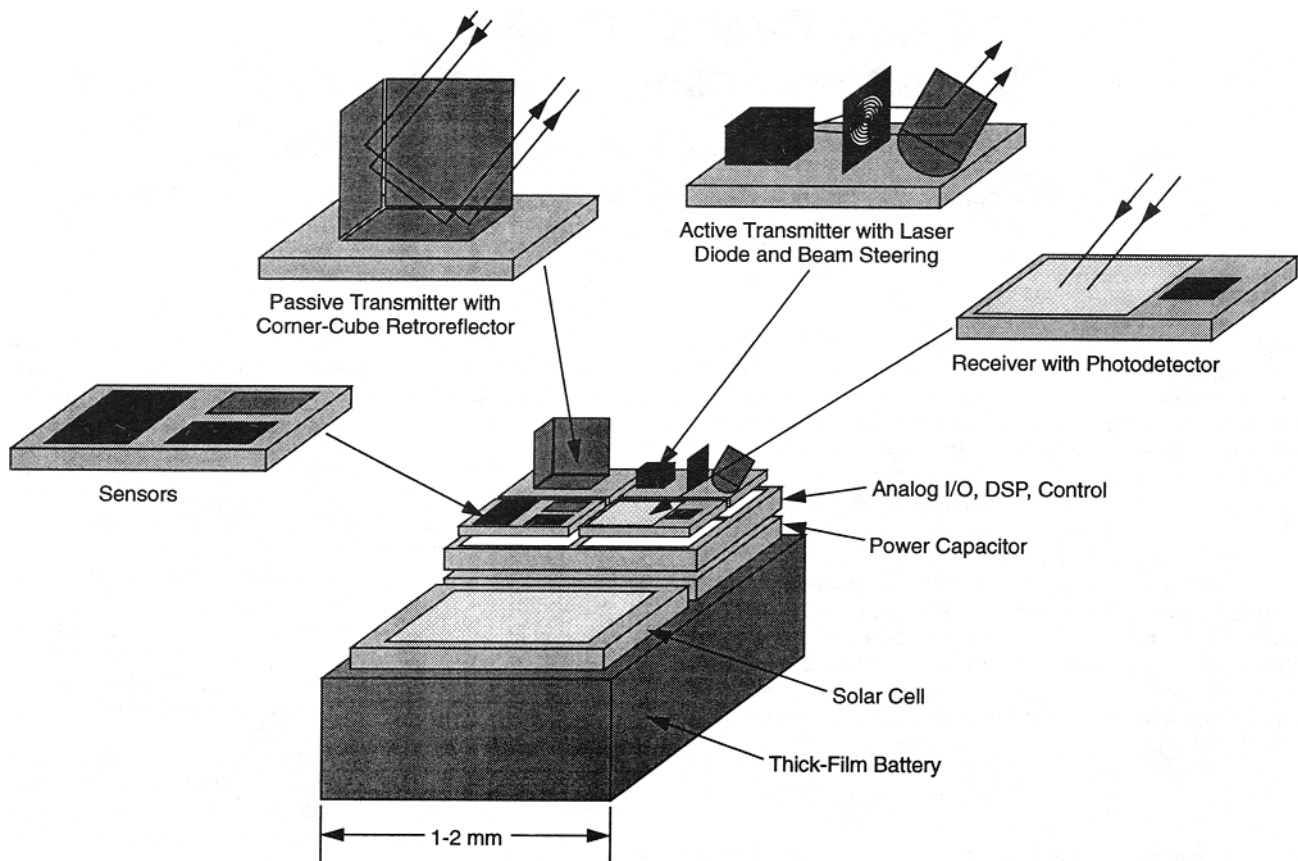
Figure 1. Smart dust mote, containing microfabricated sensors, optical receiver, passive and active optical transmitters, signal-processing and control circuitry, and power sources.
