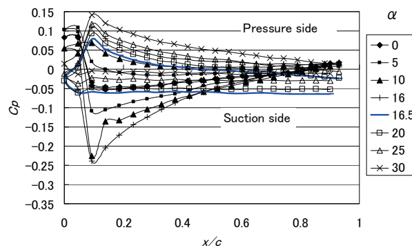
Fig. 5 C_p distributions for various angles of attack ( U = 20\text{m/s} , Plasma OFF)
