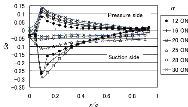
Fig. 6 C_p distributions for various angles of attack ( U = 20\text{m/s} , Plasma ON, f = 200\text{ Hz} )
