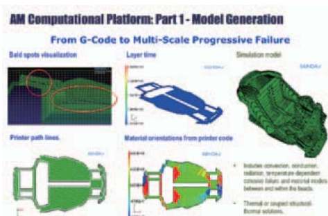
Fig. 24 3DPrinter molding process simulation
