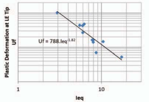
Fig. 15 Plastic deformation at LE tip vs Moment of inertia I_{eq}
