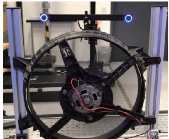
Fig. 22 Measuring object and setup for cooling fan rotation
