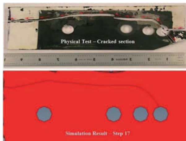
Fig. 9 Frame crack during physical test compared with simulation result obtained using full vehicle response based 3D crack growth process.
