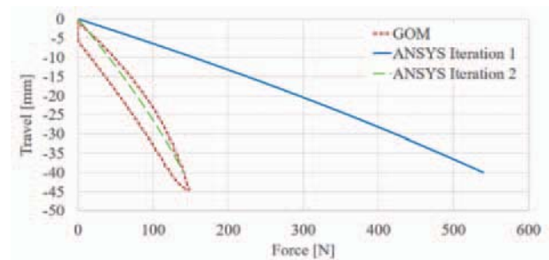
Fig. 21 Quantitative analysis of CAE optimization result using DIC measurement result.
