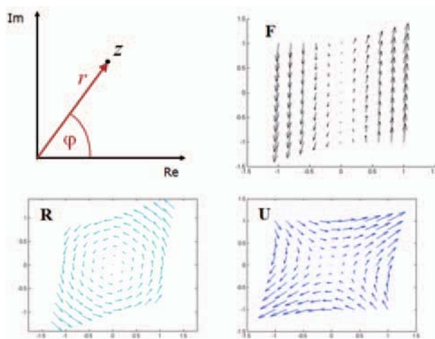
Fig. 8 Polar decomposition
