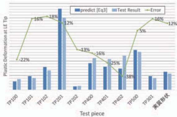
Fig. 17 Validation of predictive Equation (3)
