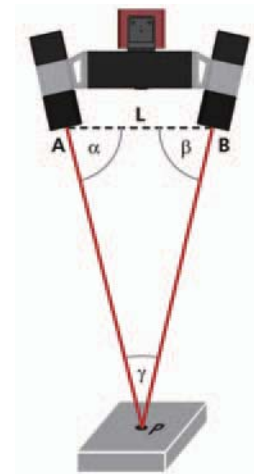
Fig. 4 Triangulation principle using 2 cameras
