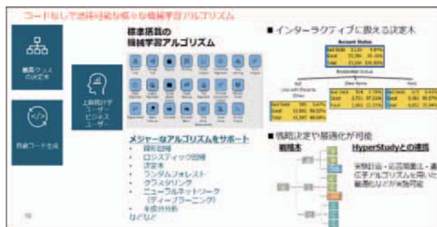
Fig. 19 Machine learning
