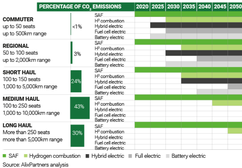
FIGURE 2: APPLICATION AND ESTIMATED COMMERCIAL AVAILABILITY OF DISRUPTIVE ENGINE TECHNOLOGIES
