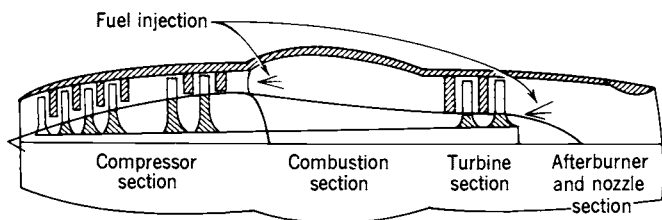
FIGURE 1-1. Simplified schematic diagram of a turbojet engine.
