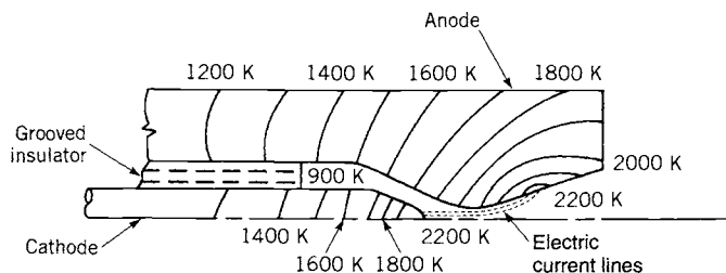
FIGURE 19-5. Typical estimated temperature distribution in the electrodes of an arcjet.
