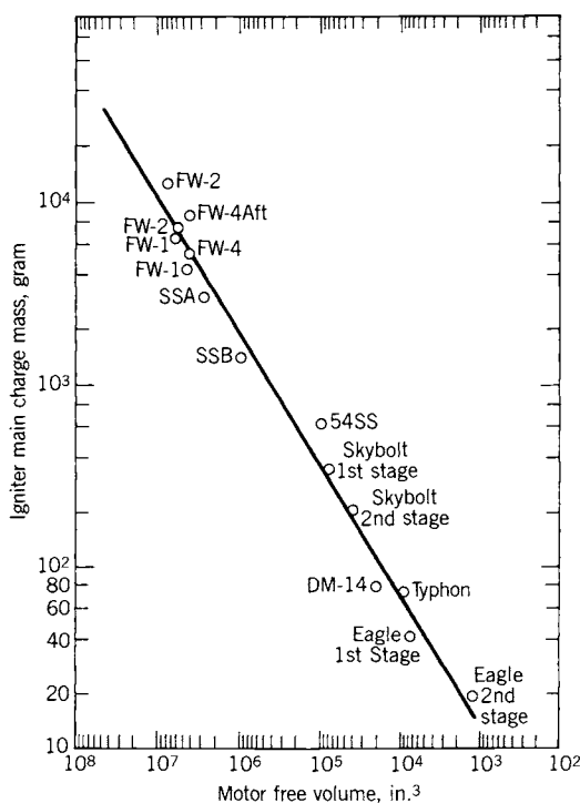
FIGURE 14-16. Igniter charge mass versus motor free volume, based on experience with various-sized rocket motors using AP/Al composite propellant. (Data with permission from Ref. 14-12.)
