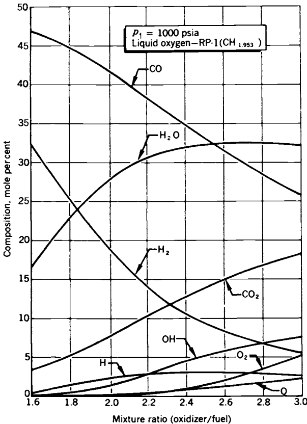
FIGURE 5-2. Calculated chamber gas composition for liquid oxygen and hydrocarbon fuel as a function of mixture ratio. Aggressive gases, such as O_2 , O , or OH , can cause oxidation of the wall materials in the chamber and the nozzle.
