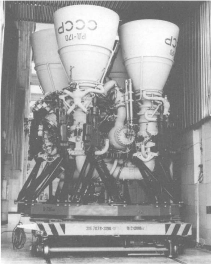
FIGURE 10-10. The RD-170 rocket engine, shown here on a transfer cart, can be used as an expendable or reusable engine (up to 10 flights). It has been used on the Zenith, Soyuz booster, and Energiya launch vehicles. The tubular structure supports the four hinged thrust chambers and its control actuators. It is the highest thrust liquid rocket engine in use today. (Courtesy of NPO Energomash, Moscow.)
