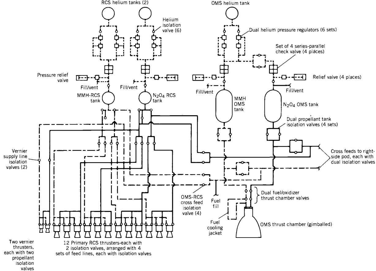
FIGURE 6-4. Simplified flow diagram of the propellant feed system flow for the left aft pod of the Orbital Maneuvering System (OMS) and Reaction Control System (RCS) of the Space Shuttle Orbiter Vehicle. Solid lines: nitrogen tetroxide ( N_2O_4 ); dash-dot lines: monomethylhydrazine (MMH); short dashed lines: high-pressure helium. (Source: NASA.)
