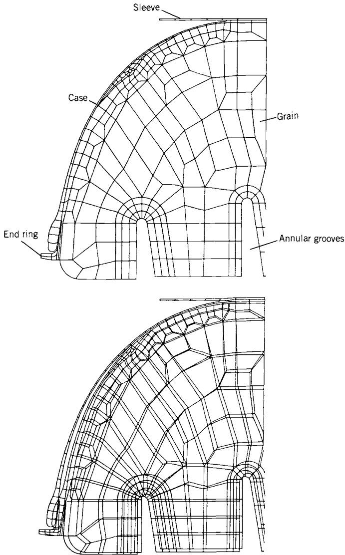
FIGURE 11-22. Finite element analysis grid of the forward end of a cast grain in a filament-wound plastic case. The grain has an internal tube and annular grooves. The top diagram shows the model grid elements and the bottom shows one calculated strain or deformation condition. (Reprinted with permission from A. Turchot, Chapter 10 of Ref. 11-1).
