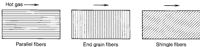
FIGURE 14–12. Simplified sketches of three different types of fiber-reinforced ablative materials.
