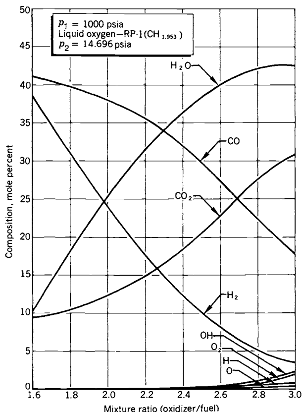
FIGURE 5-3. Calculated nozzle exit gas composition for shifting equilibrium conditions as a function of mixture ratio. Breakdown into O, OH, or H and free \text{O}_2 occurs only at the higher temperatures or higher mixture ratios.
