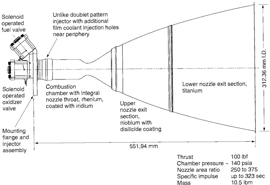
FIGURE 8–18. Radiation-cooled reaction control thruster R-4D-15 uses nitrogen tetroxide and monomethylhydrazine propellants. The large nozzle area ratio allows good vacuum performance. It has three different nozzle materials, each with a lower allowable temperature (Re 4000°F; Nb 3500°F; Ti 1300°F. (Courtesy of Kaiser-Marquardt Company.)
