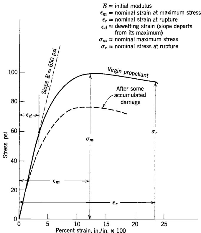
FIGURE 11-21. Stress-strain curves for a typical composite-type solid propellant showing the effect of cumulative damage. The maximum stress \sigma_m is higher than the rupture stress \sigma_r of the tensile test sample.
