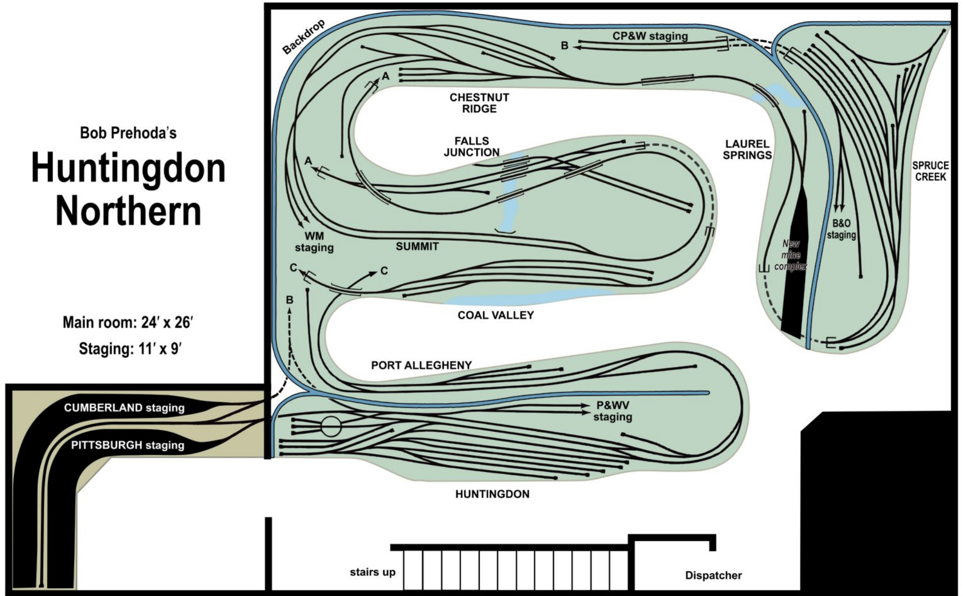
9. The Huntingdon Northern track plan.
