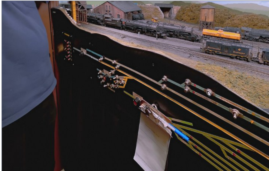
14. Stepping back from the view in [13] to show the track diagram and controls on the fascia. Bob uses the fascia as the layout control panels, which is quite effective and conserves aisle space.
