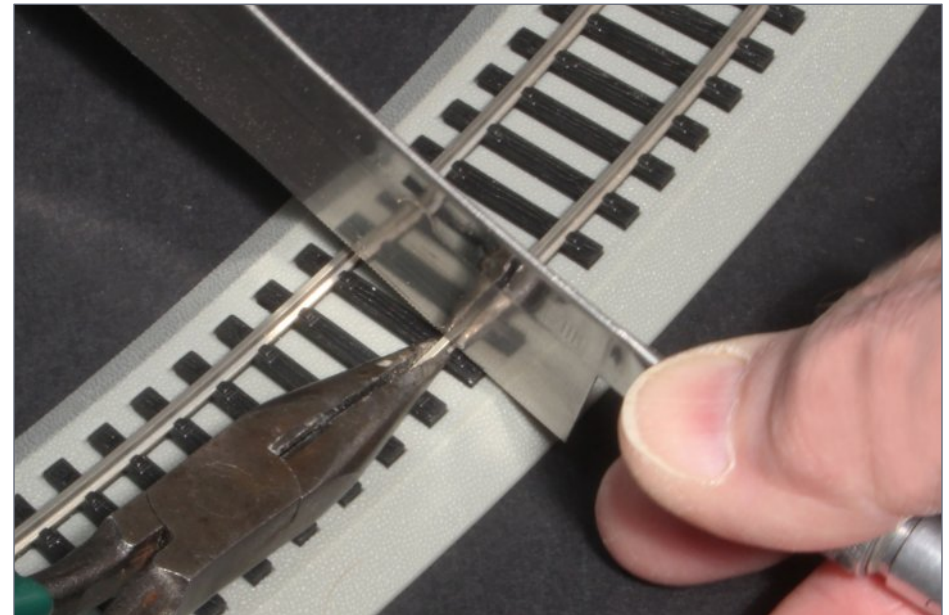
10. I used a razor saw to cut the insulating gaps in the rails. I held the rail tightly with needle-nose pliers. This reduced the risk of ripping the rail from its plastic ties. I then smoothed the tops and sides of the cuts with a rail cleaning eraser.
