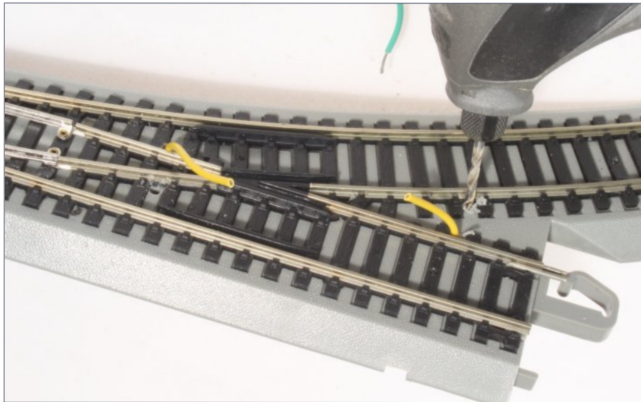
18. Drill four 1/16-inch holes to the outside of both outer rails so these yellow and green "jumper" wires can be installed.
