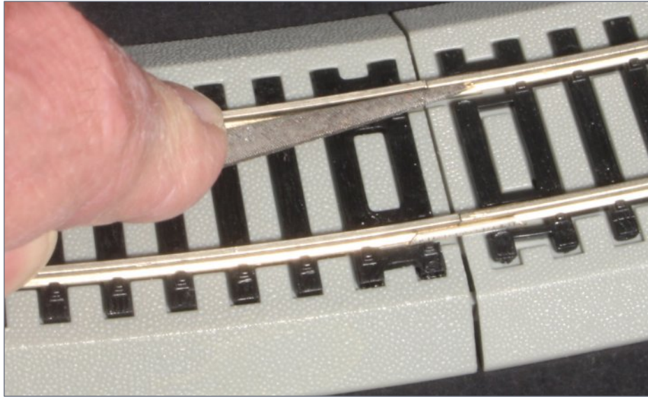
7. Cleaning up the inside of the rails with a jeweler's file.
