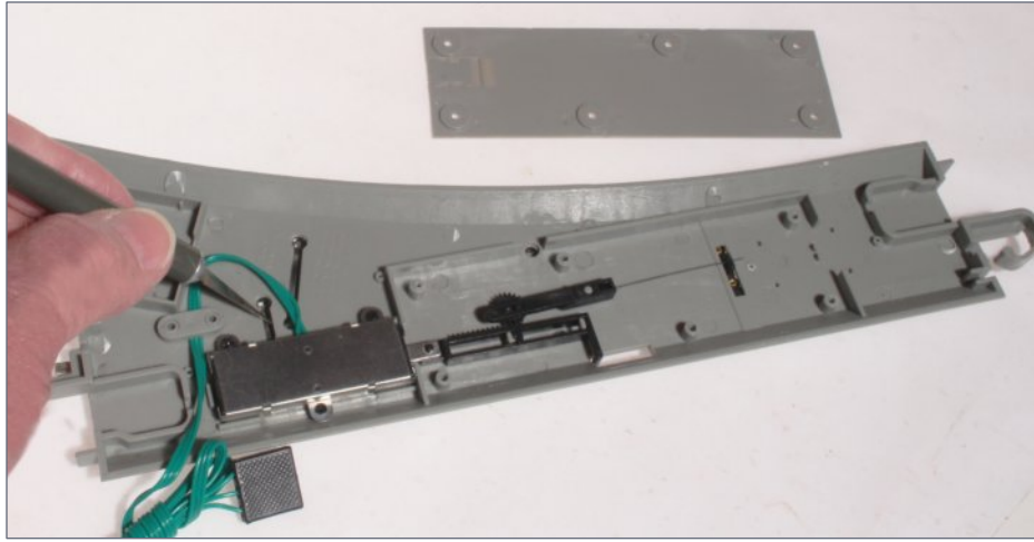
17. E-Z Track turnouts have thin copper strips on the underside that connect the rails on both sides of the frog. Use a hobby knife to cut both.
