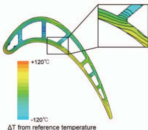
Fig. 5 Blade temperature distribution (CHT analysis)
