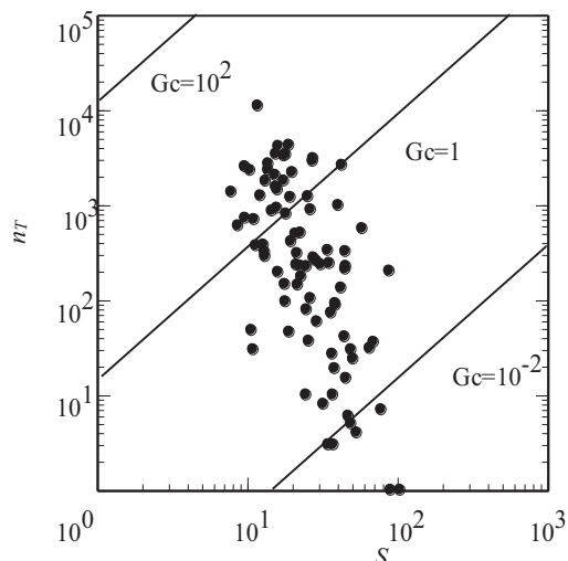
Fig. 11 G number of individual droplet clusters
