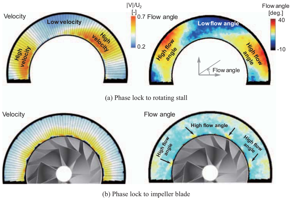
Fig. 7 Velocity and flow angle distribution at 50% span at (6)
