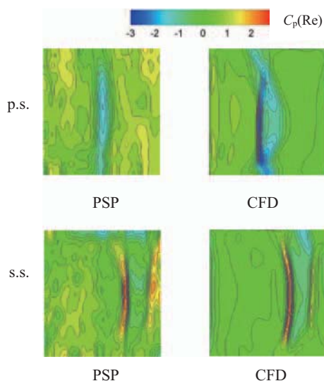
Fig. 6 Unsteady pressure distribution on blade surface (3) (PSP and CFD, Blade 0, Real part of unsteady pressure)
