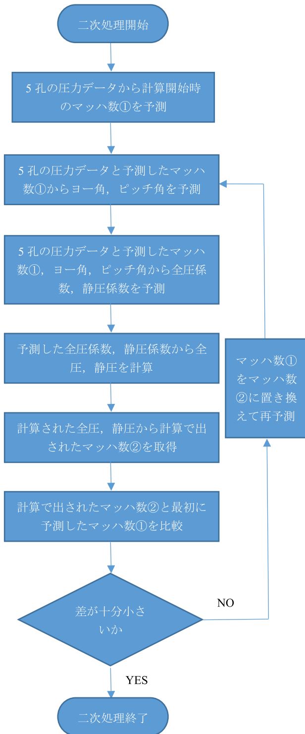
Fig. 5 Program flow chart (Validation phase)
