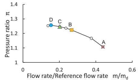
Fig. 11 Tested compressor characteristics (3)
