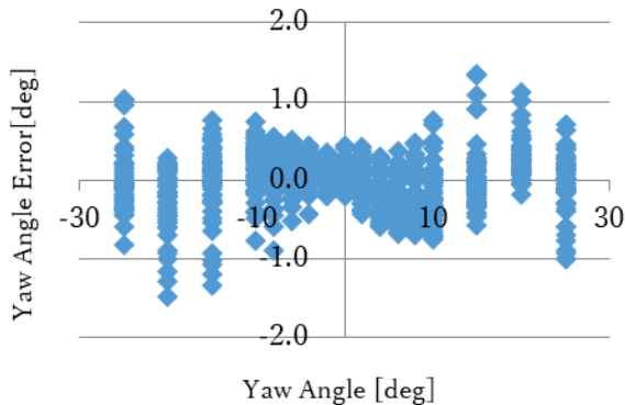
Fig. 3 Yaw angle error from curve fit method
