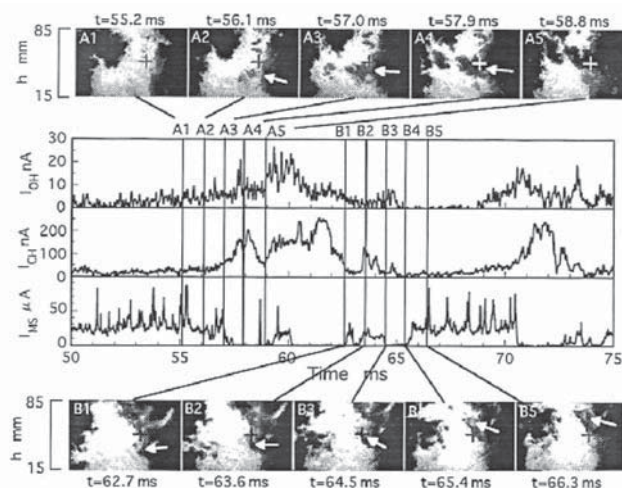
Fig. 9 Simultaneously monitored time-series data
