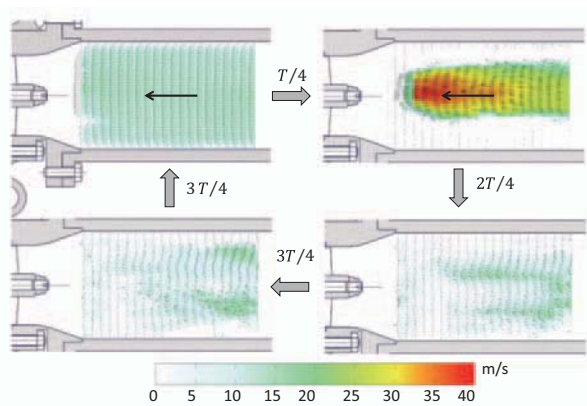
Fig. 15 Velocity vector distribution along pipe axis at surge (3)
