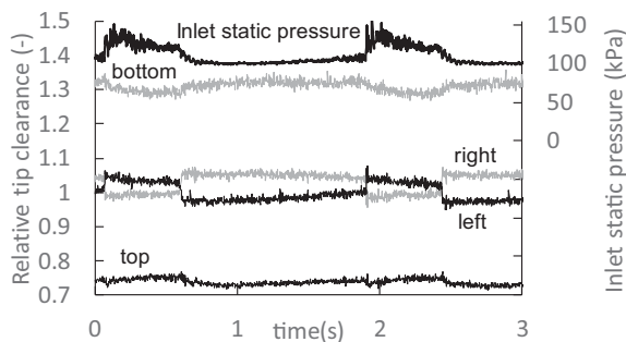
Fig. 21 Tip clearance at leading edge during surge
