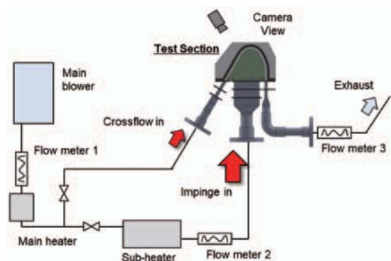
Fig. 6 Experimental system for internal cooling
