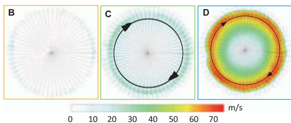
Fig. 14 Velocity vector distribution at 1.05D_2^{(3)}
