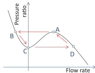
Fig. 23 Schematic of surge cycle (4)
