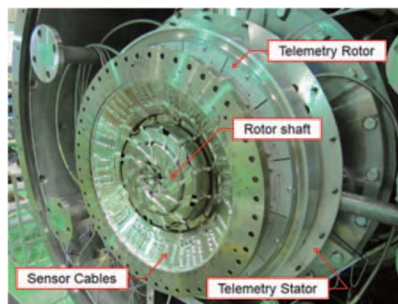
Fig. 3 Telemetry system
