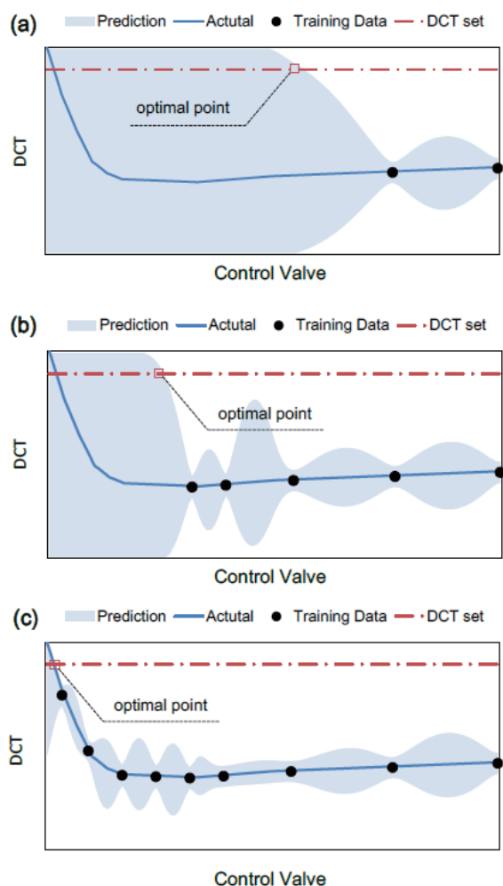
Fig. 7 Prediction result of each simulation point
