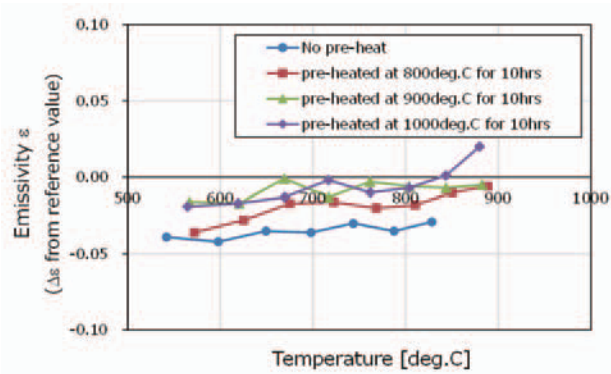
Fig. 14 Measured Emissivity
