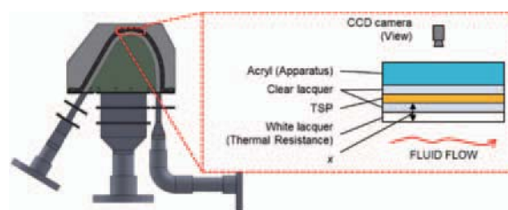
Fig. 7 Layers of paints applied
