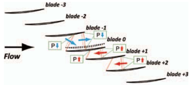
Fig. 7 Shock wave behavior responding to blade movement (3)
