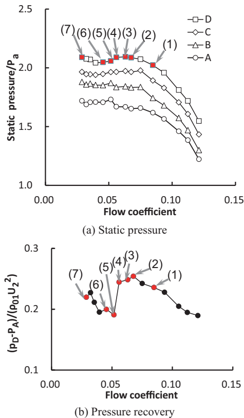
Fig. 2 Static pressure and pressure recovery in vaneless diffuser ( P_a =ambient pressure, P_A and P_D are static pressures at A and D shown in figure 1, U_2 and \rho_{01} are impeller tip velocity and stagnation density at compressor inlet) (1)
