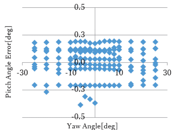
Fig. 7 Yaw angle error from machine learning, without P1 data
