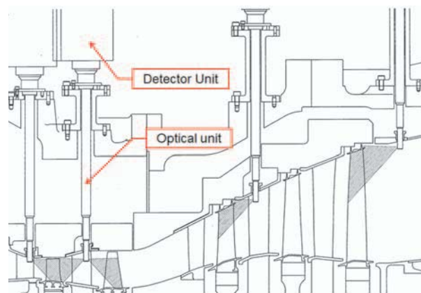
Fig. 12 Pyrometer installation
