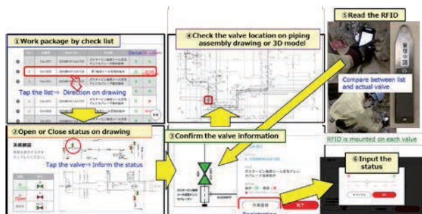
Fig. 9 Manual valve management system
