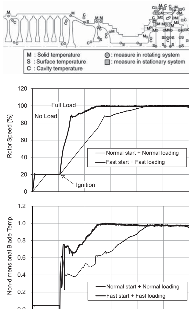
Fig. 6 Temperature measurement under transient condition
