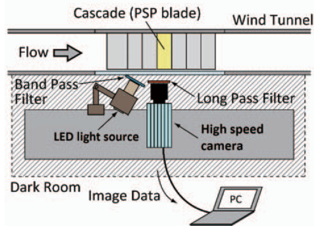
Fig. 2 PSP measurement system (3)
