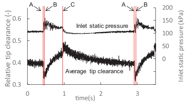
Fig. 22 Tip clearance at trailing edge during surge
