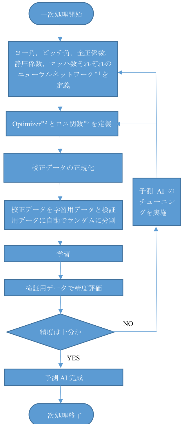
Fig. 4 Program flow chart (Learning phase)
