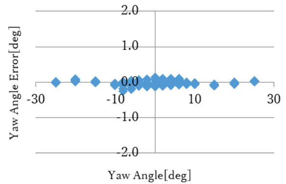
Fig. 6 Yaw angle error from machine learning method
