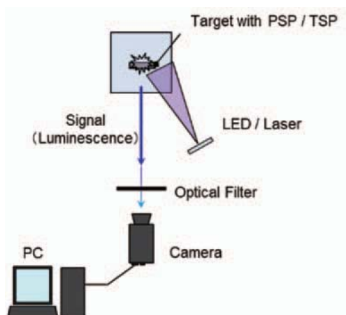
Fig. 1 Components of a measurement system in general
