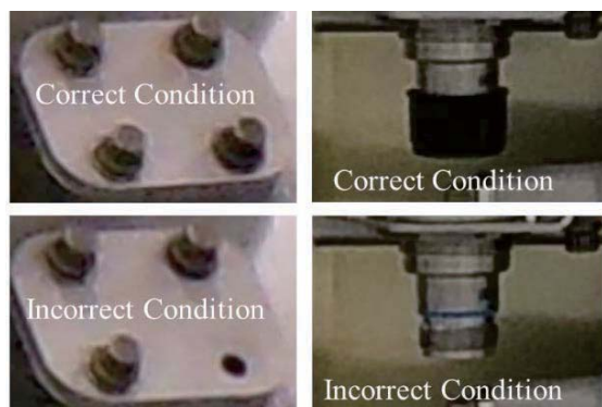
Fig. 13 Simulation of various assembly conditions
