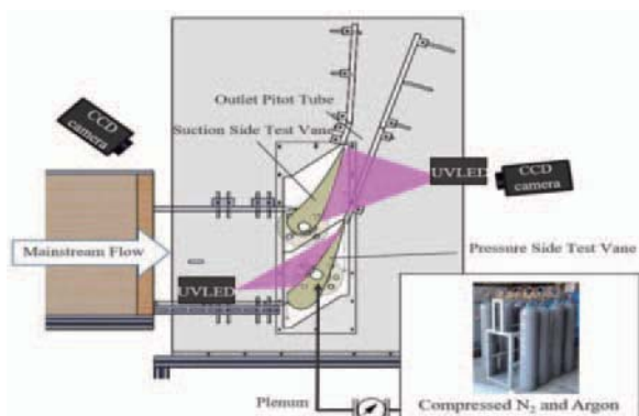
Fig. 2 Linear cascade for film cooling effectiveness measurement by use of PSP technique
