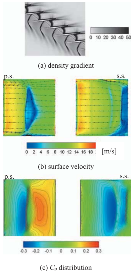
Fig. 4 CFD results of steady flow field (3)
