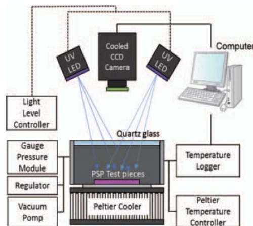
Fig. 3 A schematic of calibration setup
