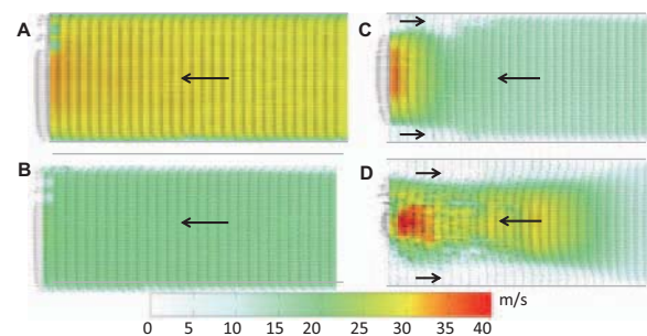
Fig. 13 Velocity vector distribution along pipe axis (3)
