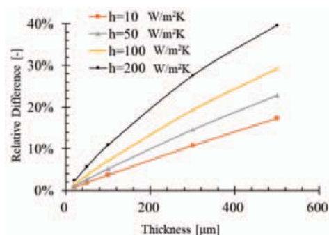
Fig. 9 Effect of thickness (relative error against the true value)
