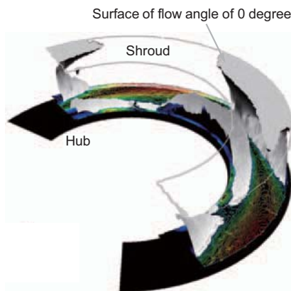
Fig. 9 Zero degree-flow angle surface (1)
