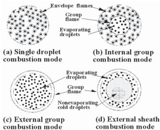
Fig. 1 Various modes of droplet group combustion
