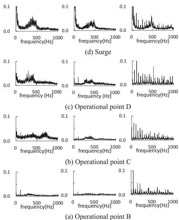
Fig. 16 FFT result at i, iii and v (left: i, middle: iii, right: v)
