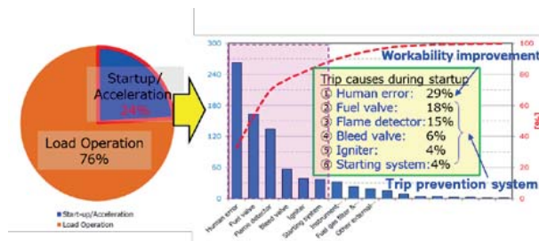
Fig. 8 Trip cause of GTCC plant
