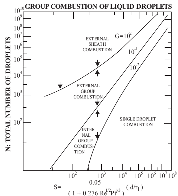
Fig. 2 Various regimes of droplet group combustion (1)
