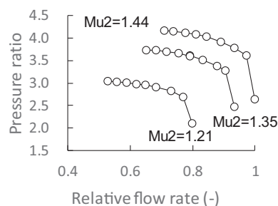
Fig. 18 Tested compressor characteristics
