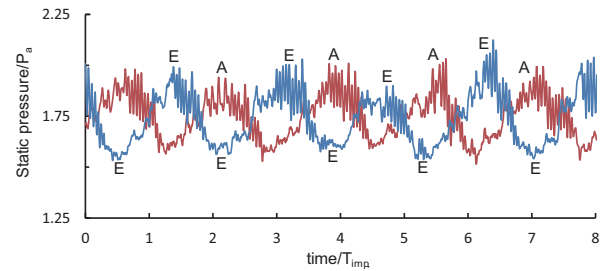
Fig. 4 Pressure signal of A and E at (6) in Fig. 2 (2)
