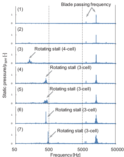
Fig. 3 Frequency of unsteady pressure and number of stall cells at different operating points (1)
