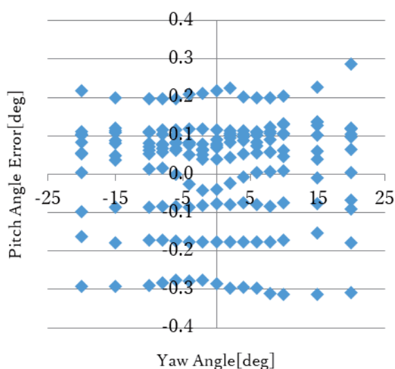
Fig. 9 Pitch angle error of 4hole probe
