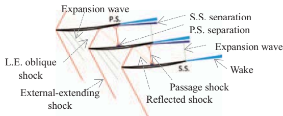
Fig. 5 Sketch of Double Shock Pattern (3)
