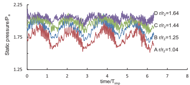
Fig. 5 Time variation of static pressure at different radius positions at (6) in Fig. 2 (2)
