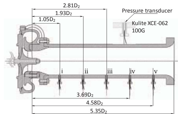
(a) Position of pressure transducer
