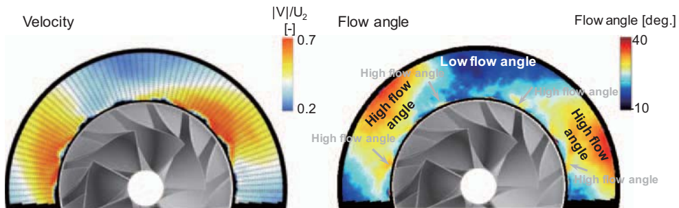
Fig. 8 Velocity and flow angle distribution at 50% span at (6) with phase lock to rotating stall and impeller blade
