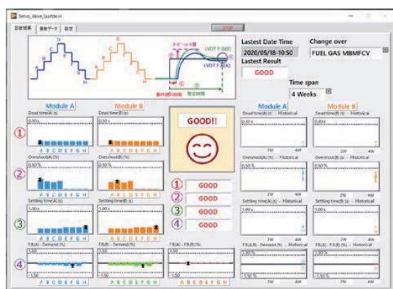
Fig. 10 GT fuel valve diagnosis
