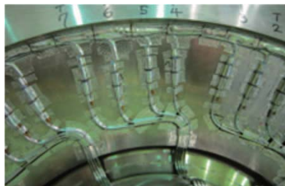
Fig. 4 Instrumentation on turbine rotor
