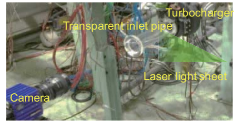
Fig. 10 Picture of test facility
