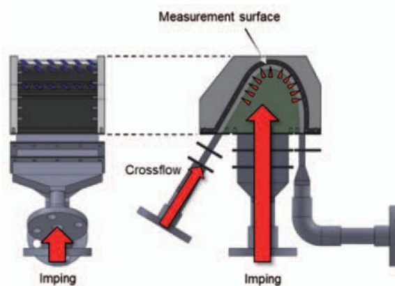
Fig. 5 Experimental apparatus for internal cooling
