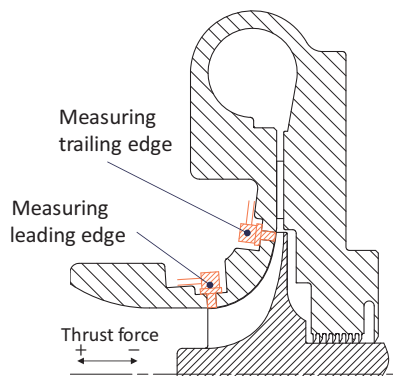
Fig. 20 Cross section of tested compressor (4)
