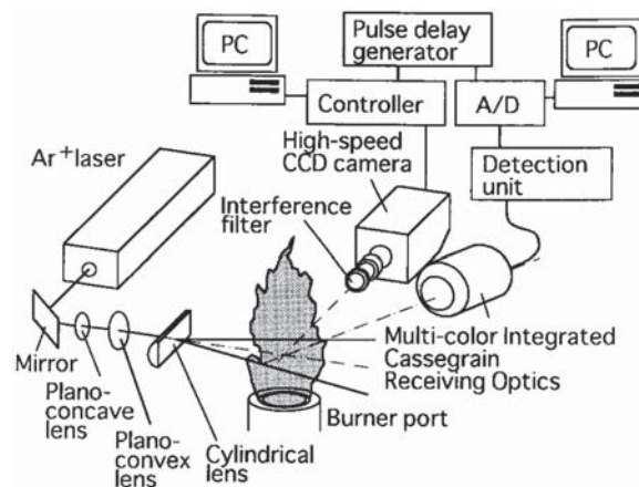
Fig. 6 Measurement system
