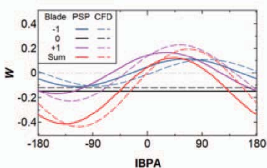
(a) W vs IBPA
