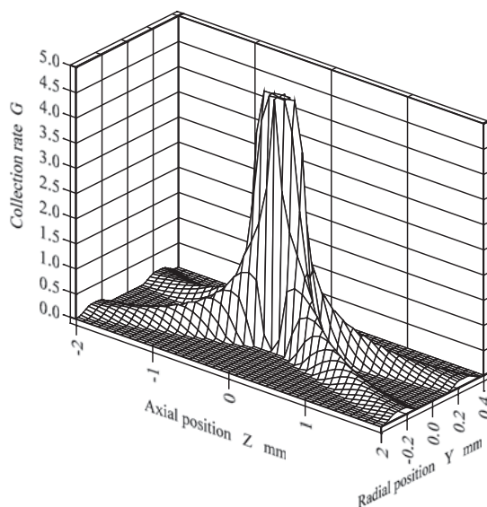
Fig. 8 Collection rate distribution of MICRO
