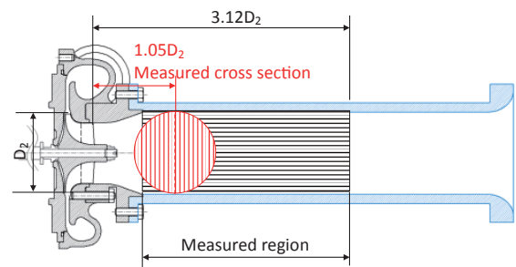
(b) Measured plane with PIV (3)
