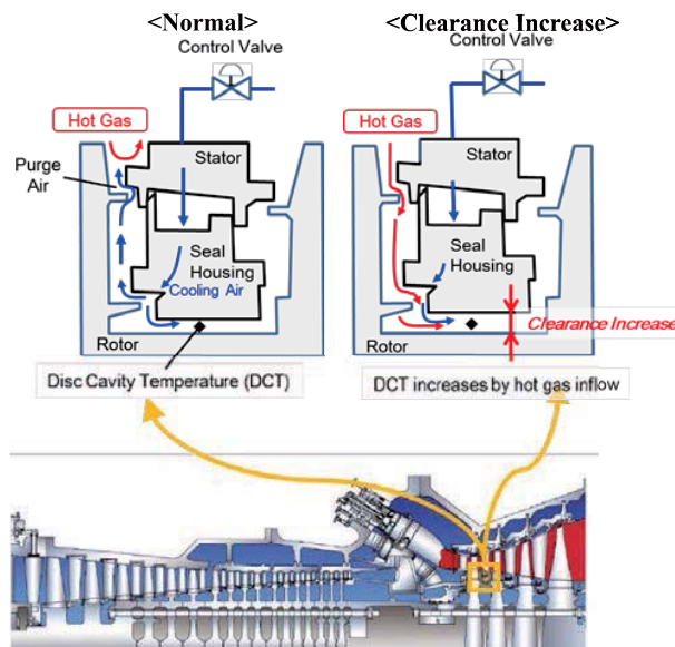
Fig. 6 Row2 turbine vane cooling air scheme
