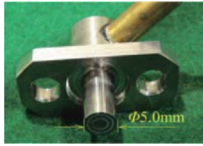
Fig. 19 Capacitive sensor (4)
