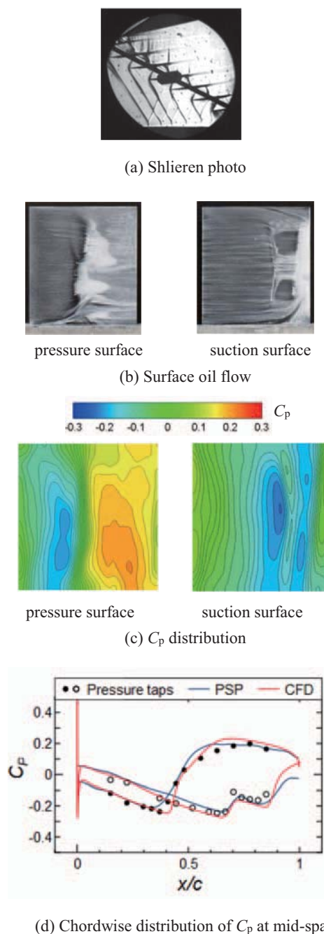
Fig. 3 Steady flow field (3)
