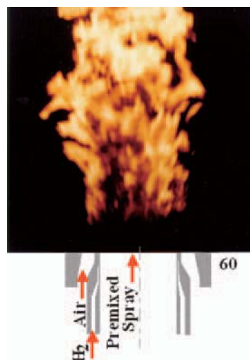
Fig. 4 Short exposure image of the flame
