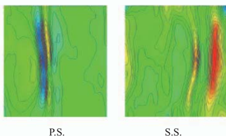
(c) Resultant W distribution on blade (PSP)
