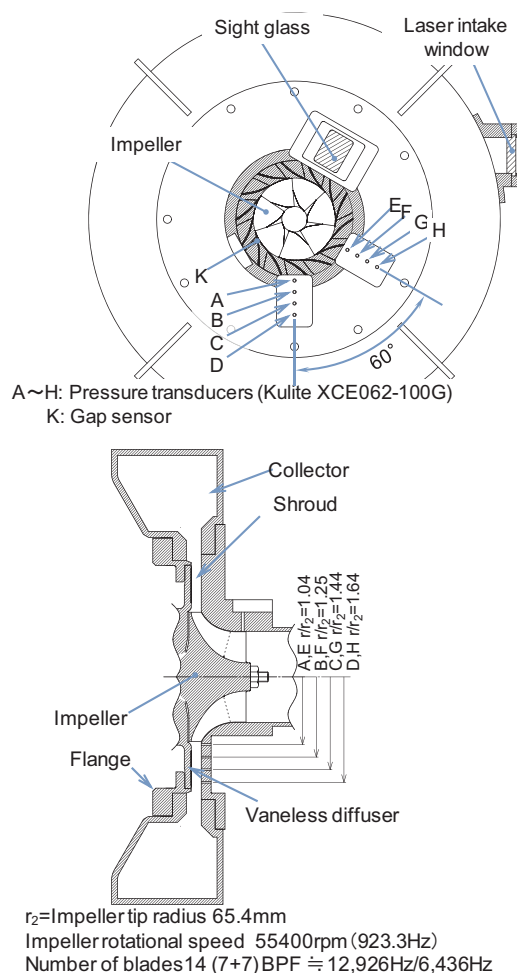
Fig. 1 Schematic of tested compressor with sensors (1)
