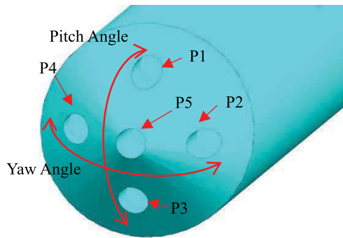
Fig. 2 5hole probe layout
