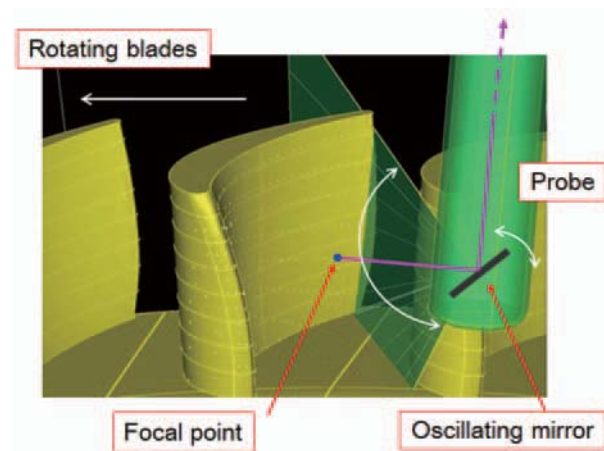
Fig. 13 Pyrometer probe
