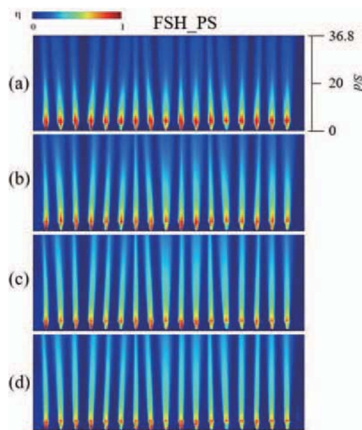
Fig. 4 Film-cooling effectiveness distributions on the pressure-side surface of the test model with fan-shaped holes ((a) BR=0.5 , (b) BR=1.0 , (c) BR=1.5 , (d) BR=2.5 )
