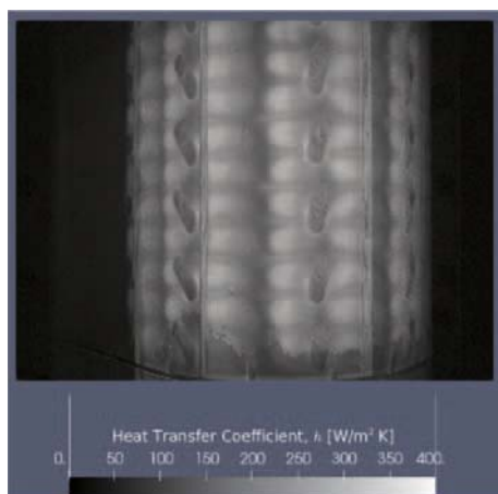
Fig. 8 Distribution of heat transfer coefficient
