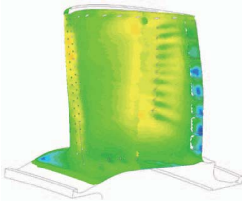
Fig. 15 Pyrometer measurement result
