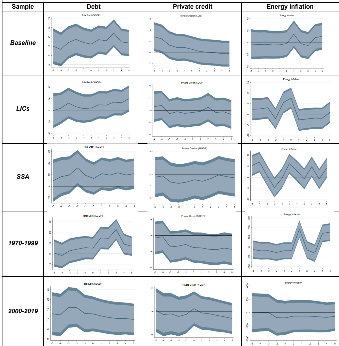
Annex Figure 4b: Event Study Results for Selected Indicators and by sub-Sample: Economic Indicators
