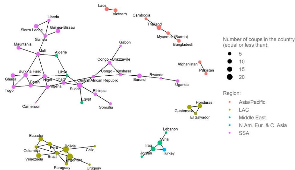
Figure 7: Spatial Correlation of Coups
