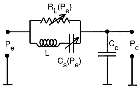
Figure 20 : "very" simplified electrical equivalent of an ear muff for low frequencies for high peak pressures
