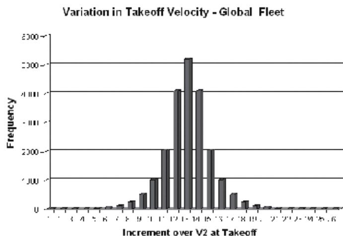
Figure 5. Example of the potential of globally pooled data in comparing aircraft operations across fleets, operators, etc.
