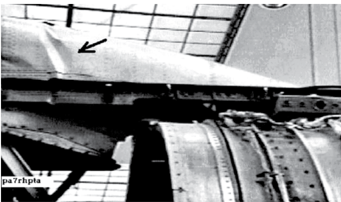
Figure 6. Pylon buckling and fractured nacelle hinges due to seizure loading.
