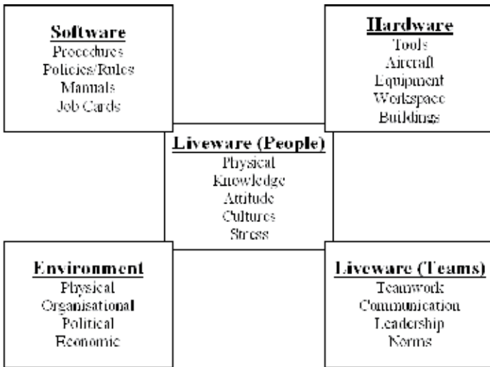
Figure 2. SHELL model.
