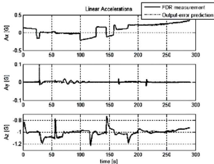
Figure 9. Simulated FDR data and output-error prediction of linear accelerations.
