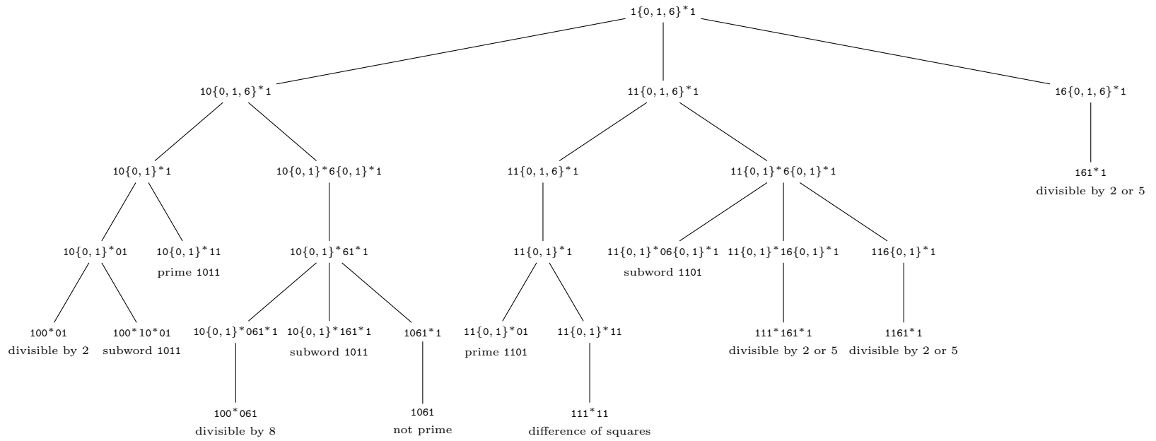
Figure 1: Tree of decompositions for 1\{0,1,6\}^*1 in base 9.
