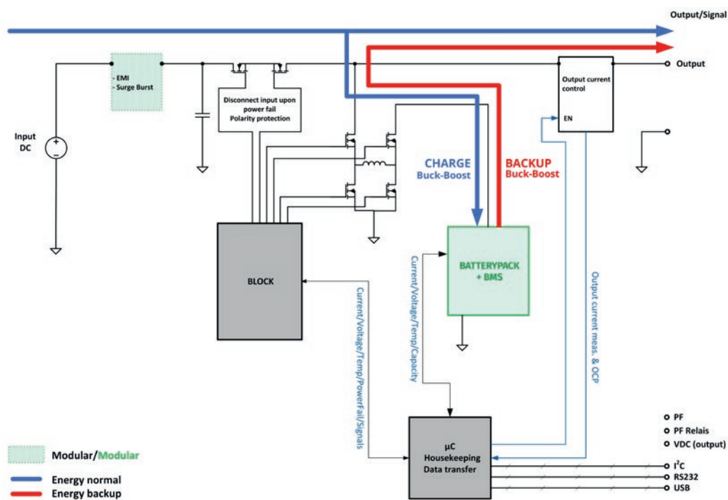
Figure 04 Block diagram DC-UPS with bidirectional buck-boost converter.
