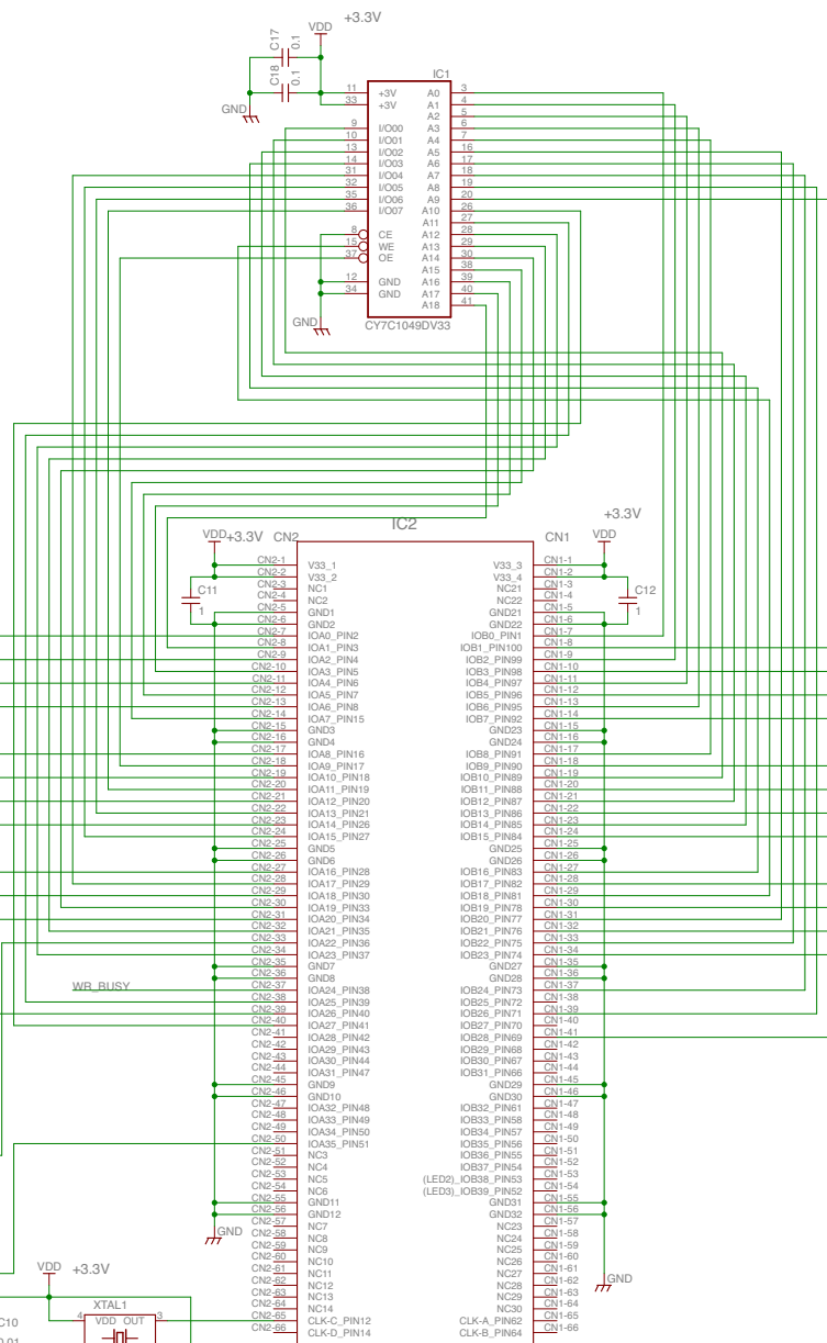
ACM-005_CPLD_BOARD Altera, MAX-II, EPM240T100C5N
