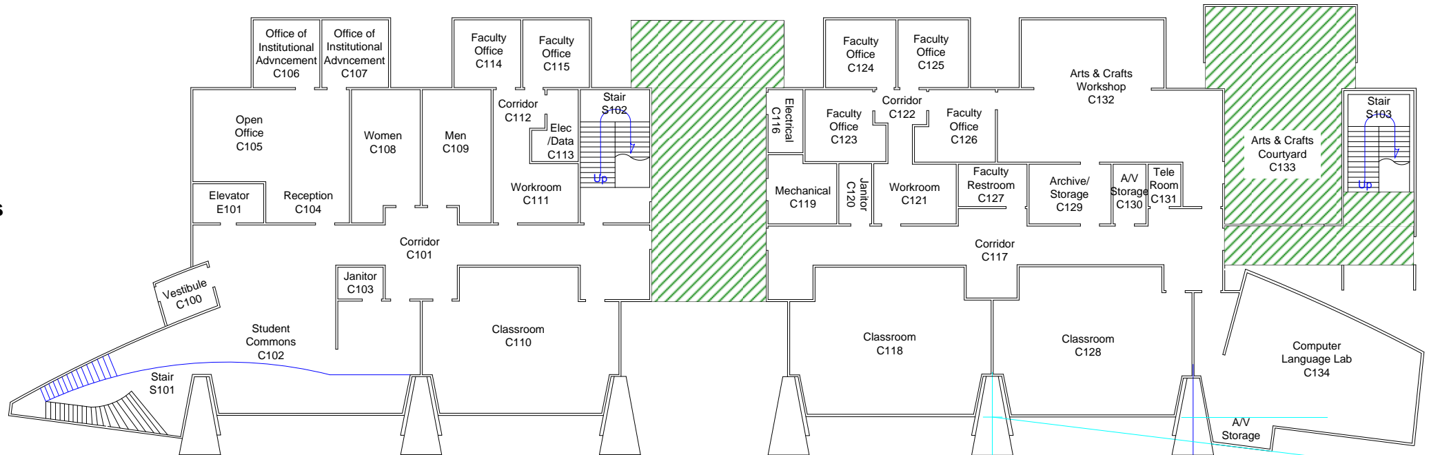
1 st Level Floor Plan
