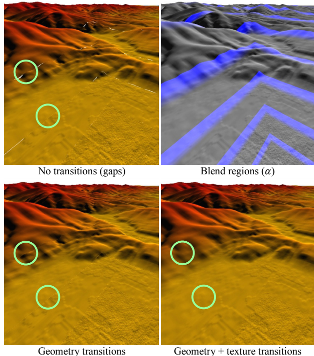
Figure 5: Visual continuity achieved with transition morphs (demonstrated with a low-resolution clipmap of size n=127 ).
