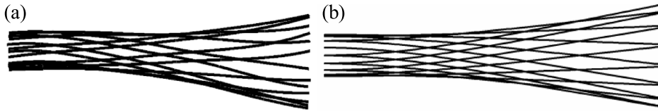
Fig. 10. Mode shape of the plate when f/f_0 = 1 obtained from the experiment (a) (Paraz et al., 2014) and current numerical simulation (b).
