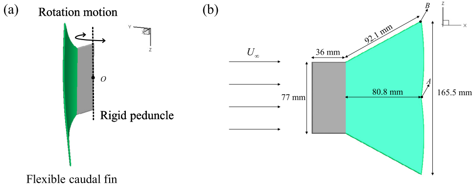
Fig. 1. Illustration of the fish caudal peduncle-fin model (a) and xz view of the model and dimensions (b).
