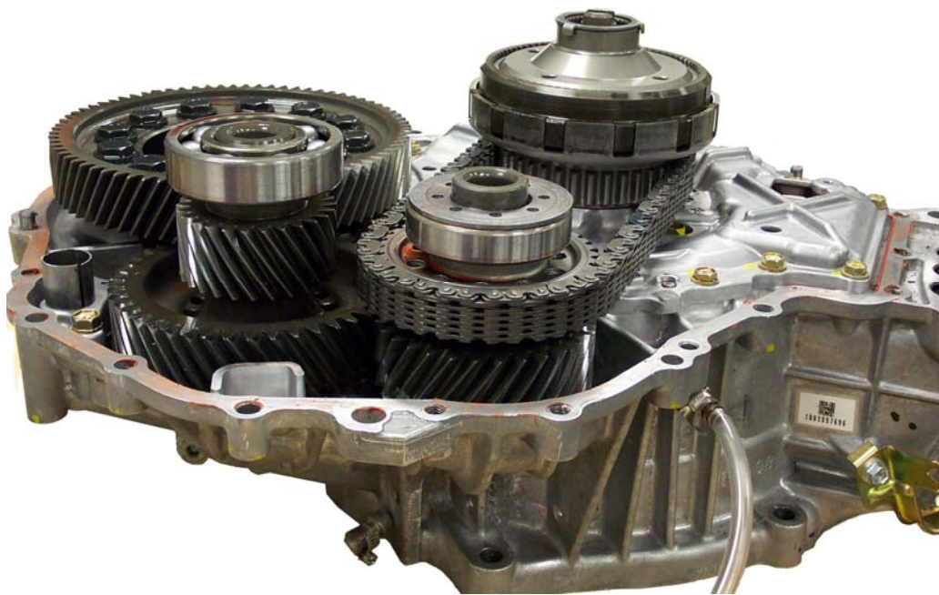
Fig. I.6. Toyota/Prius hybrid-drive transmission assembly.
