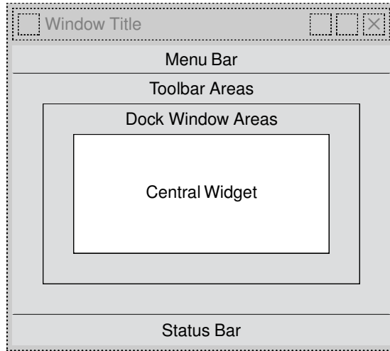
Figure 6.3 QMainWindow's areas
