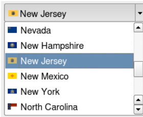
QComboBox
