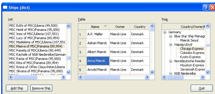
Figure 14.2 QListView , QTableView , and QTreeView in action
