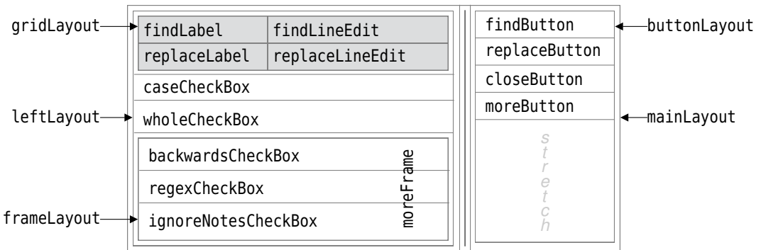
Figure 9.4 The Find and Replace dialog's layout
