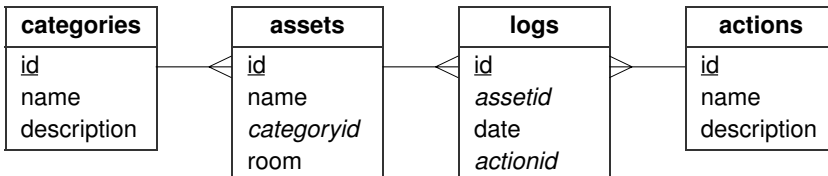
Figure 15.4 The Asset Manager database design
