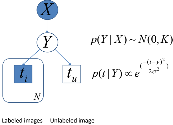
Figure 2. Graphical models in plate notation for classification via Gaussian Processes. The rounds and squares represent continuous and discrete random variables, respectively. A filled (unfilled) round/square denotes that the random variable is fully observed (unobserved). \mathbf{X} = \{\mathbf{x}_1, \dots, \mathbf{x}_n, \mathbf{x}_u\} is the set of all images and is observed for both labeled and unlabeled data points. The corresponding \mathbf{Y} = \{y_1, \dots, y_n, y_u\} is completely unobserved and the labels \{t_1, \dots, t_n\} are observed only for the training images \{\mathbf{x}_i, \dots, \mathbf{x}_n\} and unobserved for the unlabeled image \mathbf{x}_u .
