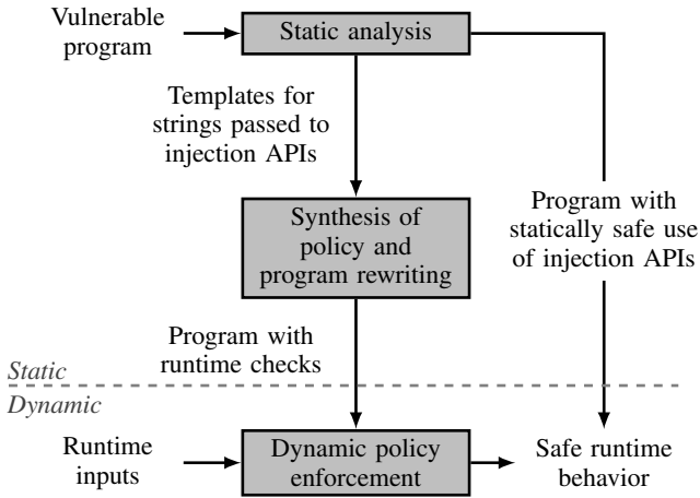
Fig. 8: Architectural diagram for mitigating injection attacks.
