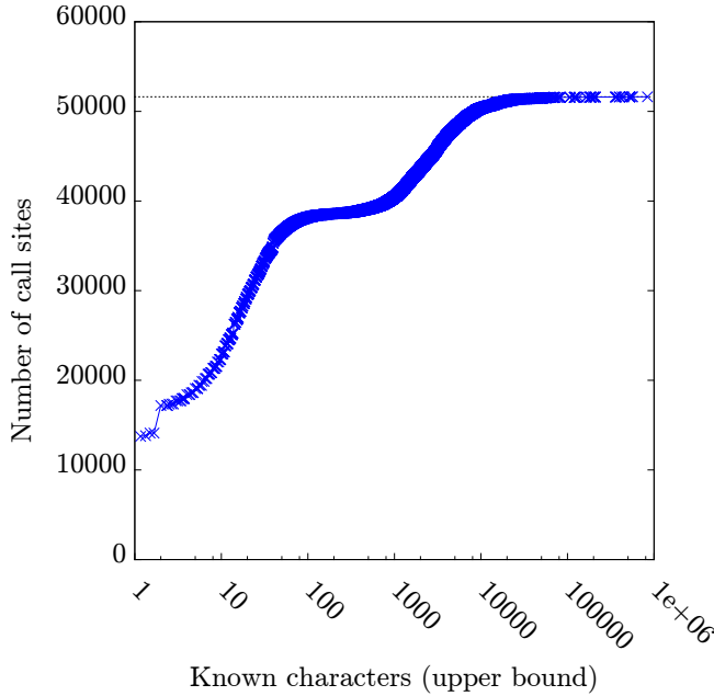
Fig. 14: CDF for the average number of constant characters per call site. Note the logarithmic horizontal axis.
