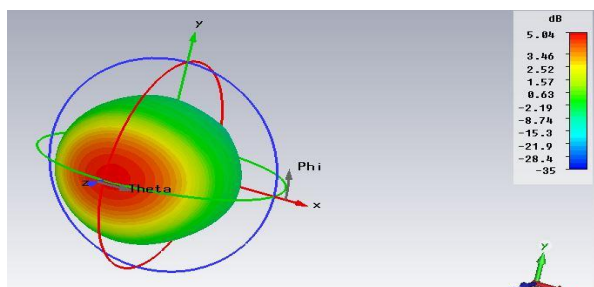
FFig 11 : EFMSSPA 3D Gain Pattern with twin slots
