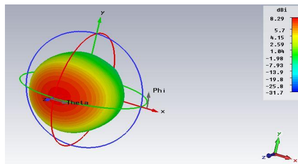
Fig 13: EFMSSPA Directivity Pattern with twin slots
