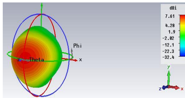
Fig 12: EFMSSPA Directivity Pattern with twin slots
