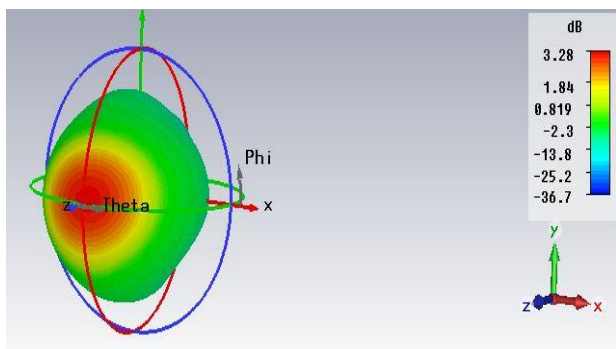
Fig 10: EFMSSPA 3D Gain pattern with twin slots
