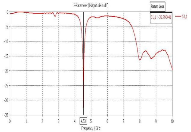
Fig 5. Return loss (S11) of EFMSSPA with twin slots
