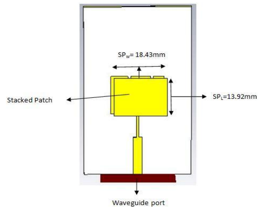
Fig 3. Edge feed Micro Strip Stacked Patch Antenna(EFMSSPA)with twin slots
