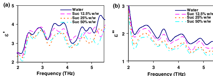
Fig. 4 The variation of dielectric function with varying concentration of sucrose. (a) The real part and (b) imaginary part.
