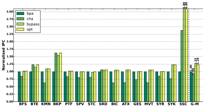
Figure 5.12: 16KB L1 cache bypassing on Fermi GPU.
