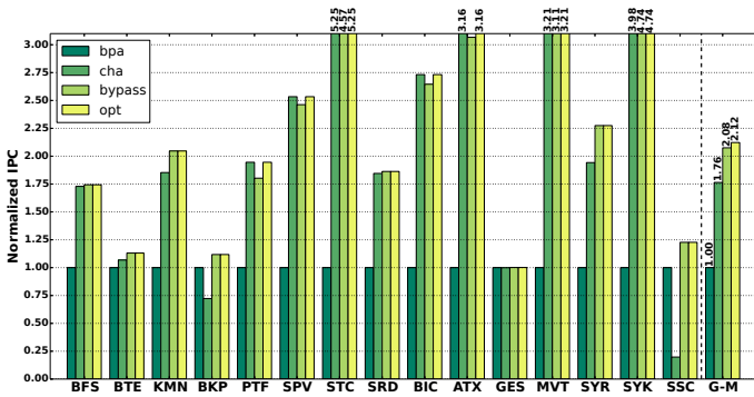
Figure 5.14: L2 cache bypassing on Fermi GPU.
