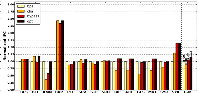
Figure 5.17: 48KB L1 cache bypassing on Kepler GPU.
