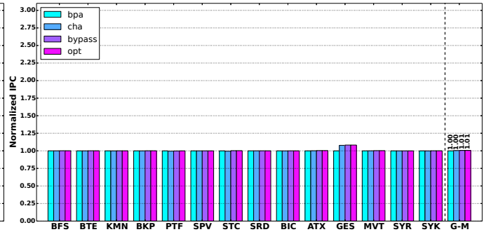
Figure 5.21: L2 cache bypassing on Maxwell GPU.
