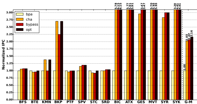
Figure 5.18: Read-only cache bypassing on Kepler GPU.
