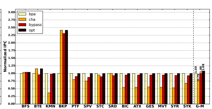
Figure 5.15: 16KB L1 cache bypassing on Kepler GPU.
