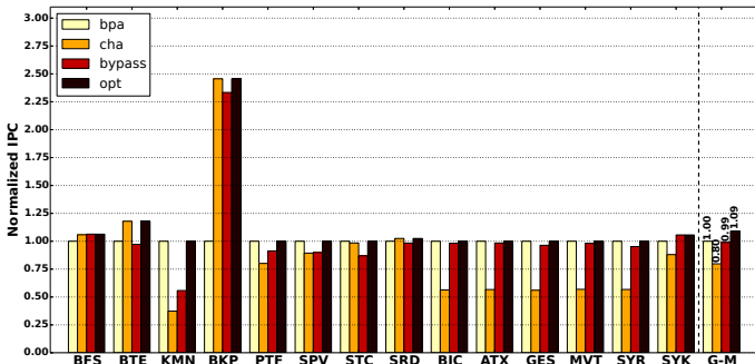
Figure 5.16: 32KB L1 cache bypassing on Kepler GPU.
