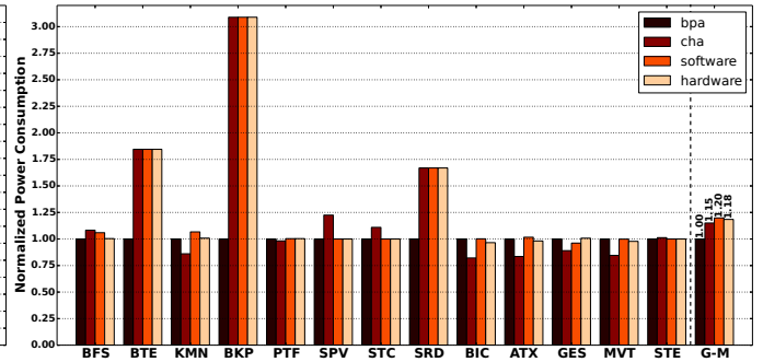
Figure 5.38: Simulation Results for Power.
