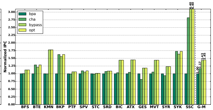
Figure 5.13: 48KB L1 cache bypassing on Fermi GPU.
