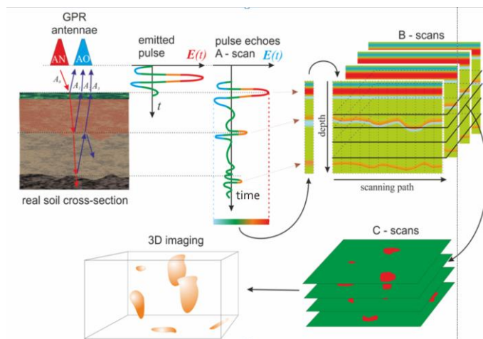
Fig. 8. Different kind of GPR imaging formation.
