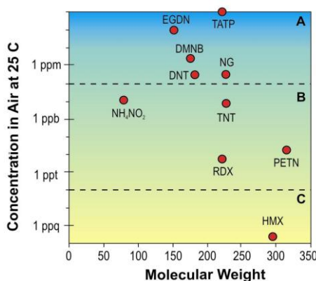
Fig. 1. Vapor concentration of explosives (A, B and C - high, medium and low respectively).
