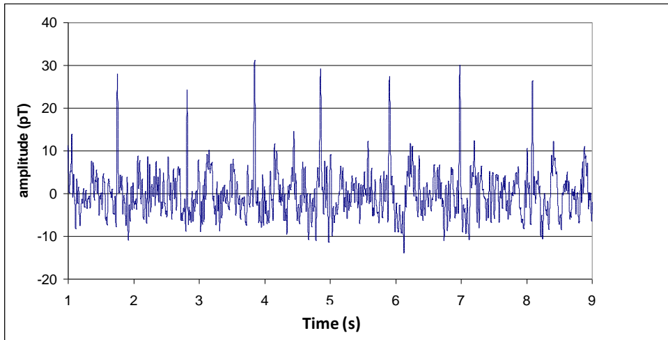
Figure 24 : Raw MCG signal recorded on a Nb-mixed sensor with a thermal noise of 100 fT/√Hz.
