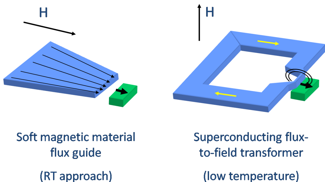
Figure 6: Flux transformers. Left: soft magnetic flux guide (room temperature approach); Right: superconducting flux transformer. The field sensor element is shown in green.
