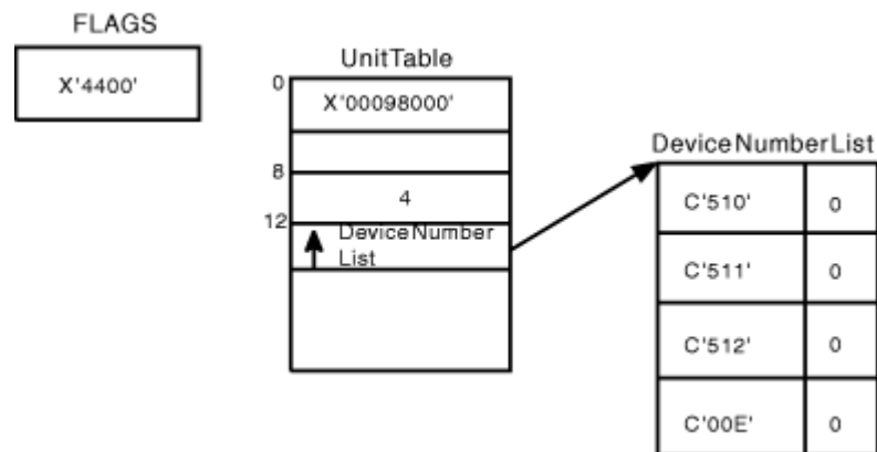
Figure 141: Input for Function Codes 1 and 5
