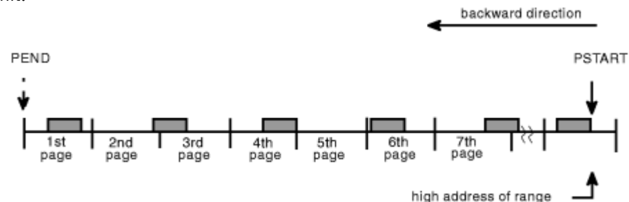
Figure 92: Illustration of Backward Direction in a Reference Pattern
