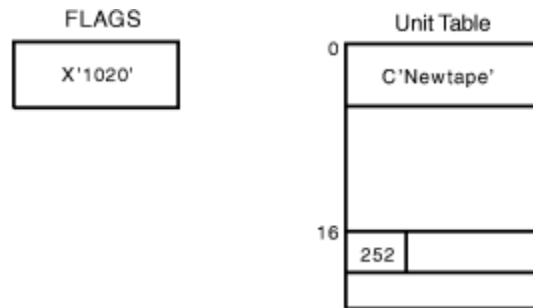
Figure 139: Input for Function Codes 3 and 10
