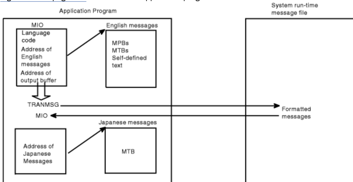
Figure 107: Using the TRANMSG Macro
