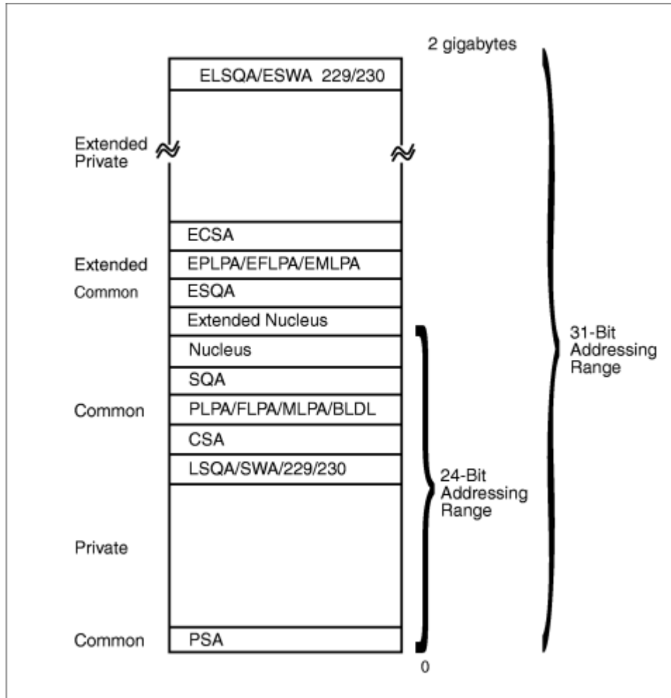
Figure 29: Two Gigabyte Virtual Storage Map
