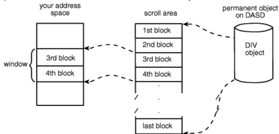
Figure 81: Mapping a Permanent Object That Has A Scroll Area
