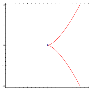
図 7: a = 0
