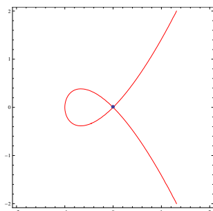
図 6: a = -1
