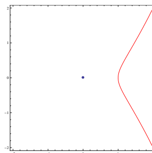
図 8: a = 1
