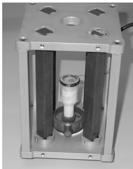
Figure 2-24: Simple Halbach structure with poor homogeneity and low field provides a sensitive volume easy to access [68].
