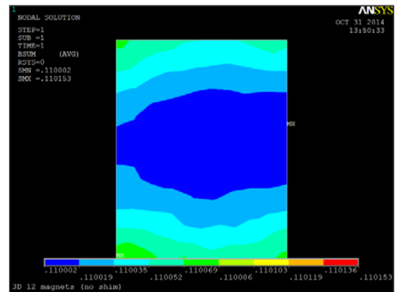
(b) Magnetic field distribution in XOY plane (5 x 6.4mm)
