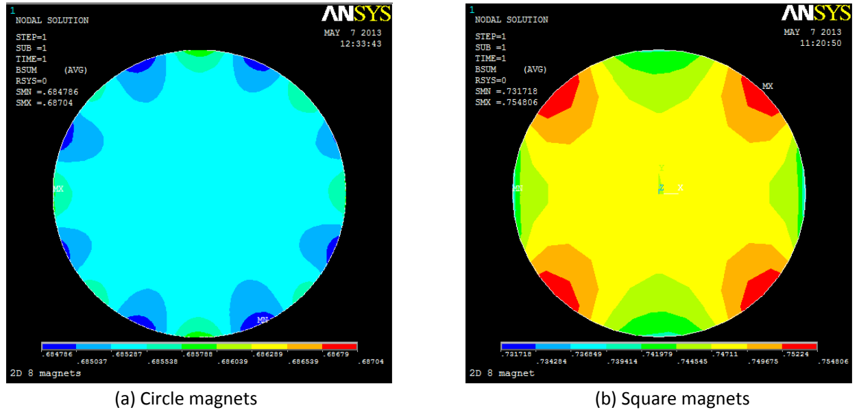
Figure 5-7: The field distribution in the region of interest 50mm diameter with n=8 .
