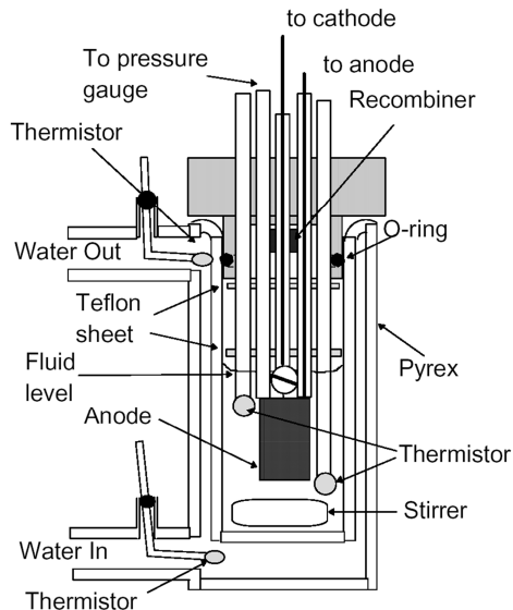
Figure 1.5. Cell and flow cooling water jacket from the calorimeter shown in Figure 1.4.
